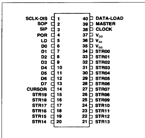
10939 Pin Configuration
