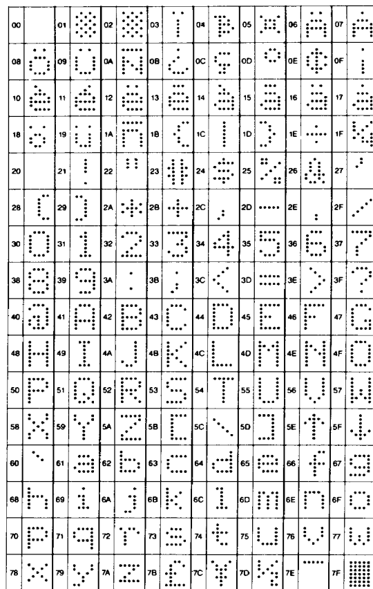
Figure 1. 5 x 7 Dot Matrix PLA Patterns
