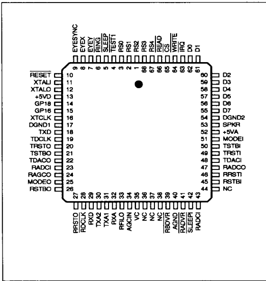
Figure 3. RC9624DP Pin Signals
