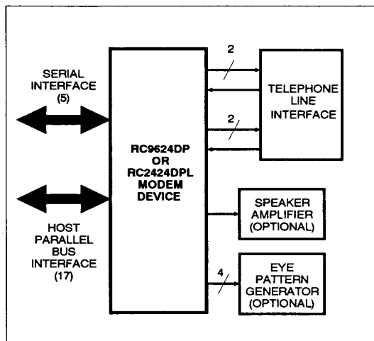
Figure 1. RC9624DP or RC2424DPL Modem General
