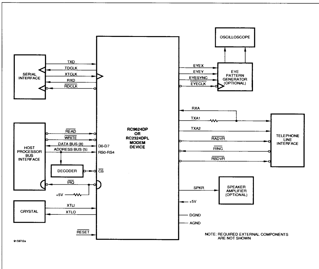
Figure 2. RC9624DP Functional Interface Signals
