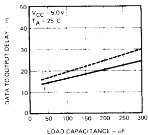
Data to Output Delay Versus Load Capacitance
