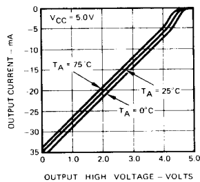
Output Current Versus Output HIGH Voltage
