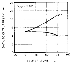
Data to Output Delay Versus Temperature
