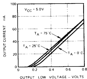
Output Current Versus Output LOW Voltage
