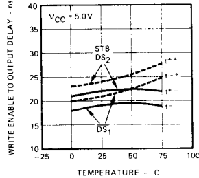
Write Enable to Output Delay Versus Temperature
