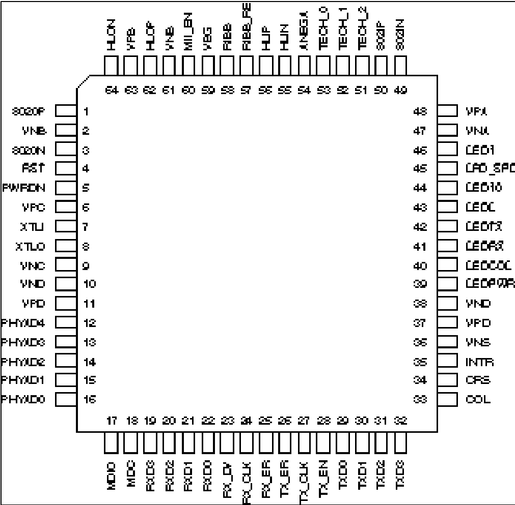
64-Lead Thin Quad Flatpack 78Q2132
