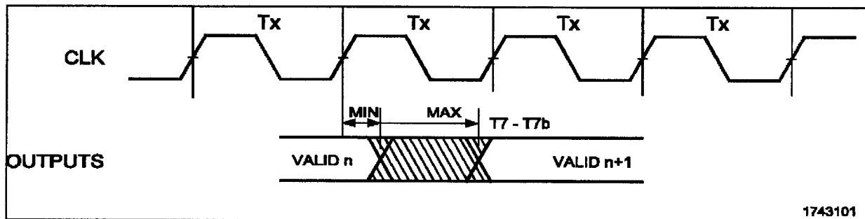
Figure 2.3. Output Valid Delay Timing
