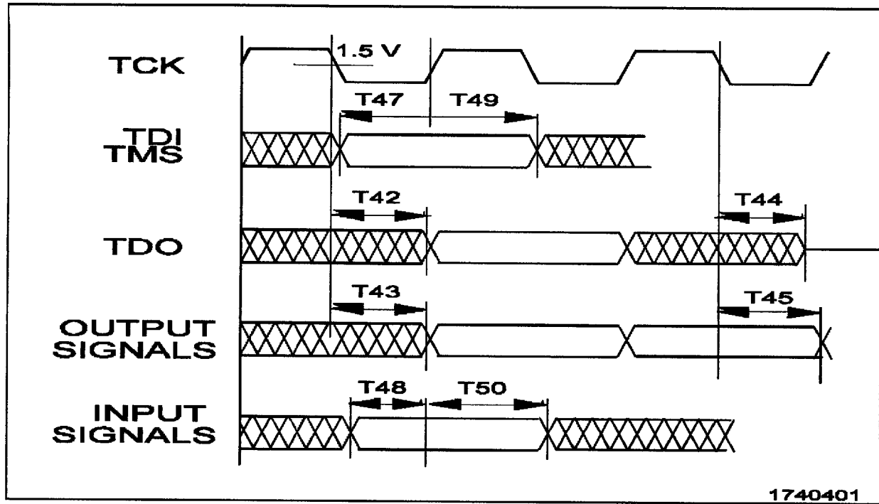
Figure 2.7. JTAG Test Timings
