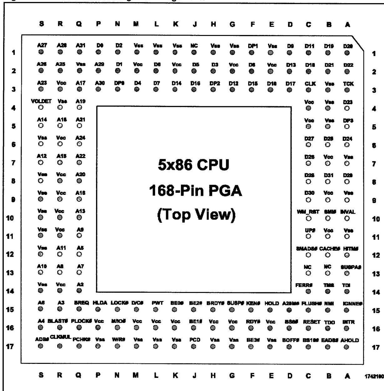
Figure 3.1. 168-Pin PGA Package Pin Assignments
