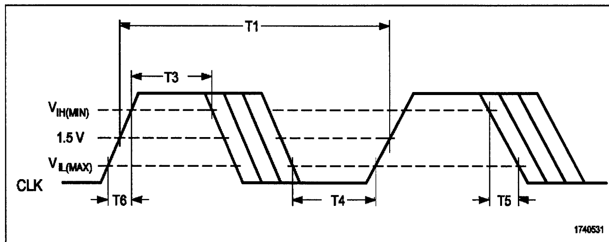
Figure 2.2. CLK Timing and Measurement Points
