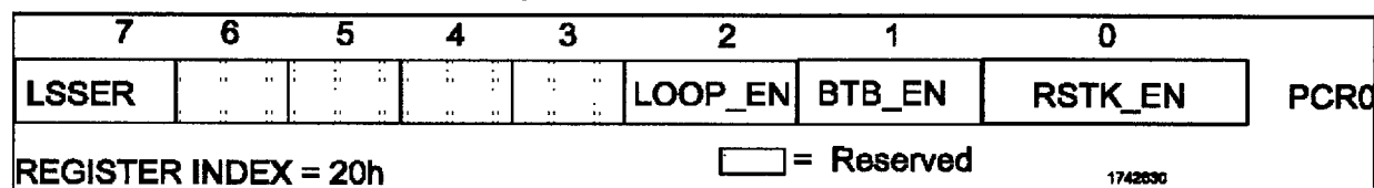
Figure 1.2. Performance Control Register 0 (PCR0)
