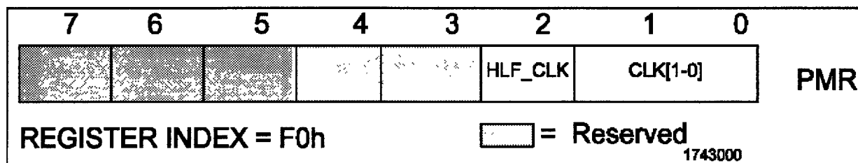
Figure 1.7. Power Management Register (PMR)
