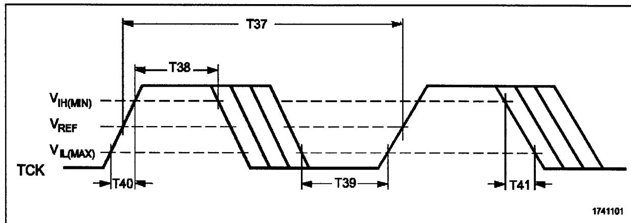
Figure 2.6. TCK Timing and Measurement Points
