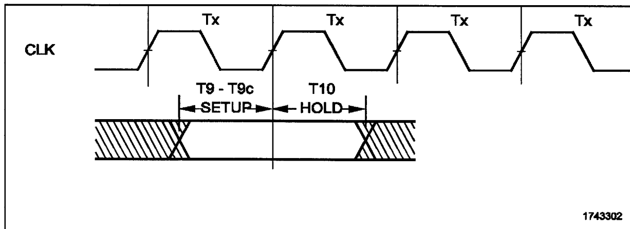
Figure 2.5. Input Setup and Hold Timing
