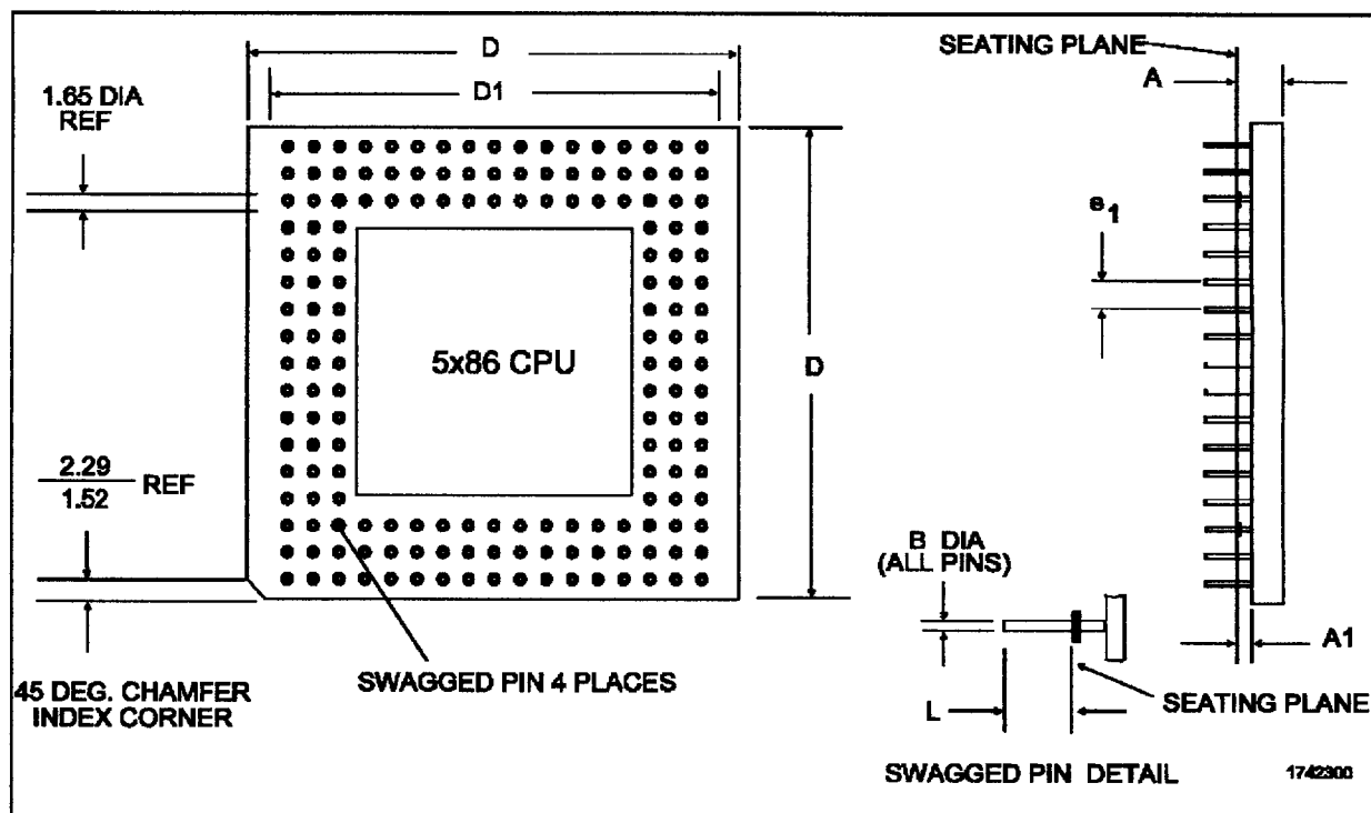
Figure 3.2. 168-Pin PGA Package
