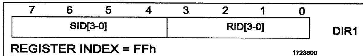
Figure 1.10. Device Identification Register 1 (DIR1)
