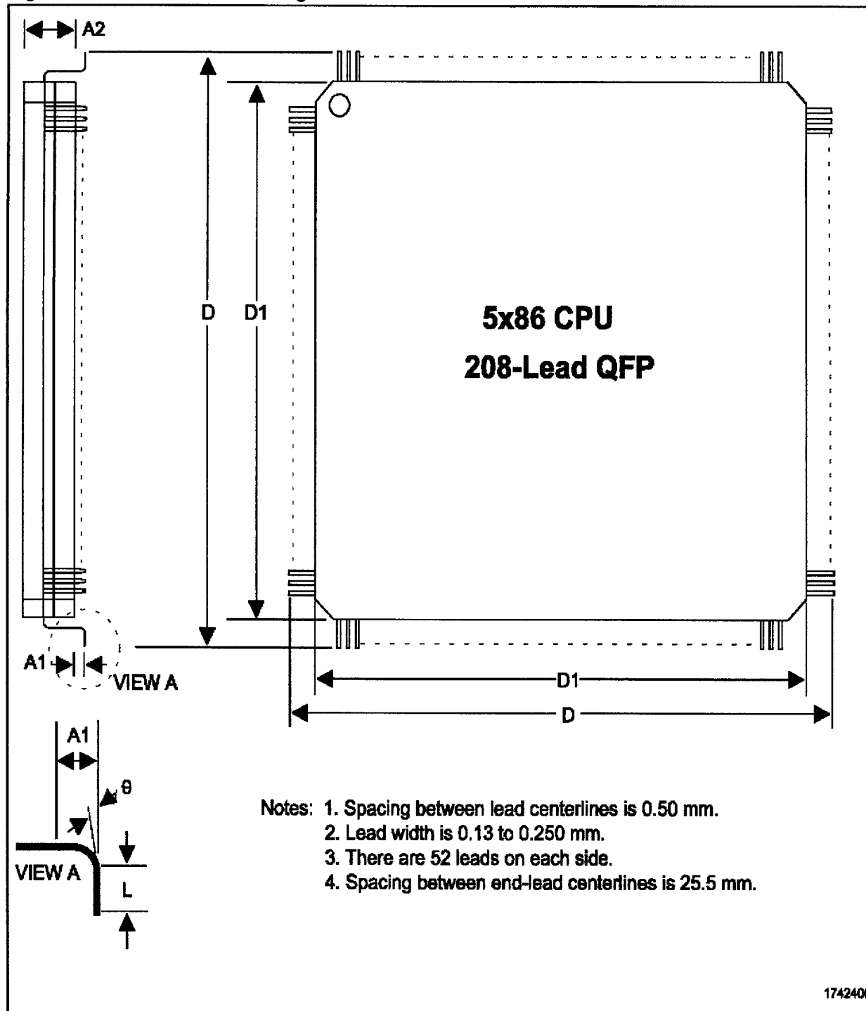
Figure 3.4. 208-Lead QFP Package
