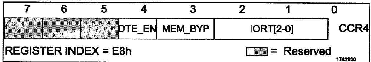
Figure 1.6. Configuration Control Register 4 (CCR4)
