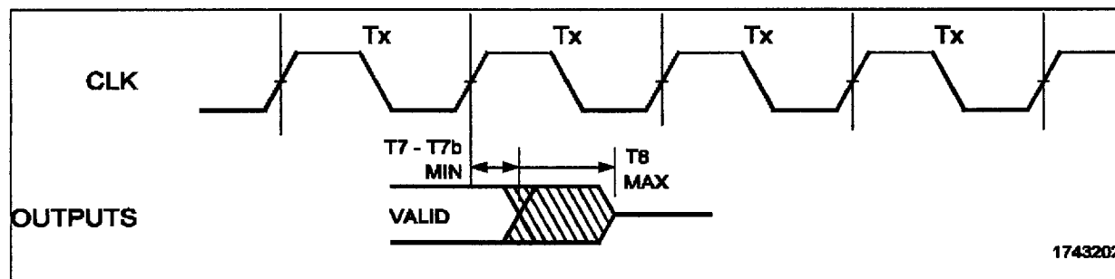
Figure 2.4. Output Float Delay Timing
