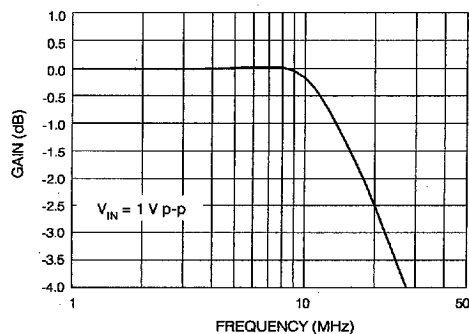
Fig. 3 Full Power Bandwidth
