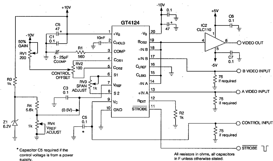
Fig. 1 Test Circuit
