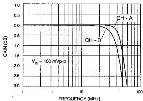
Fig. 2 Gain vs Frequency
