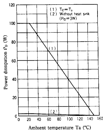
P_D - T_a
