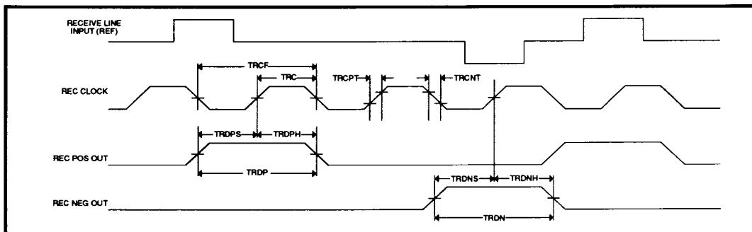
FIGURE 2: Receive Waveforms
