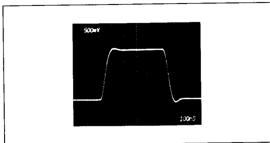
FIGURE 7: Pulse Response of Compensated X10 Amplifier in Figure 6, V_{IN} = 100mV_{p-p} , V_{OUT} = 1V_{p-p} , Frequency of Square Wave = 1MHz, C_{LOAD} = 1000pF
