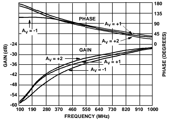
HIGH FREQUENCY REVERSE ISOLATION ( S_{12} )
