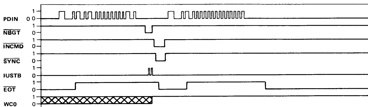
FIGURE 16. SYNCHRONIZE (NO DATA) MODE COMMAND
