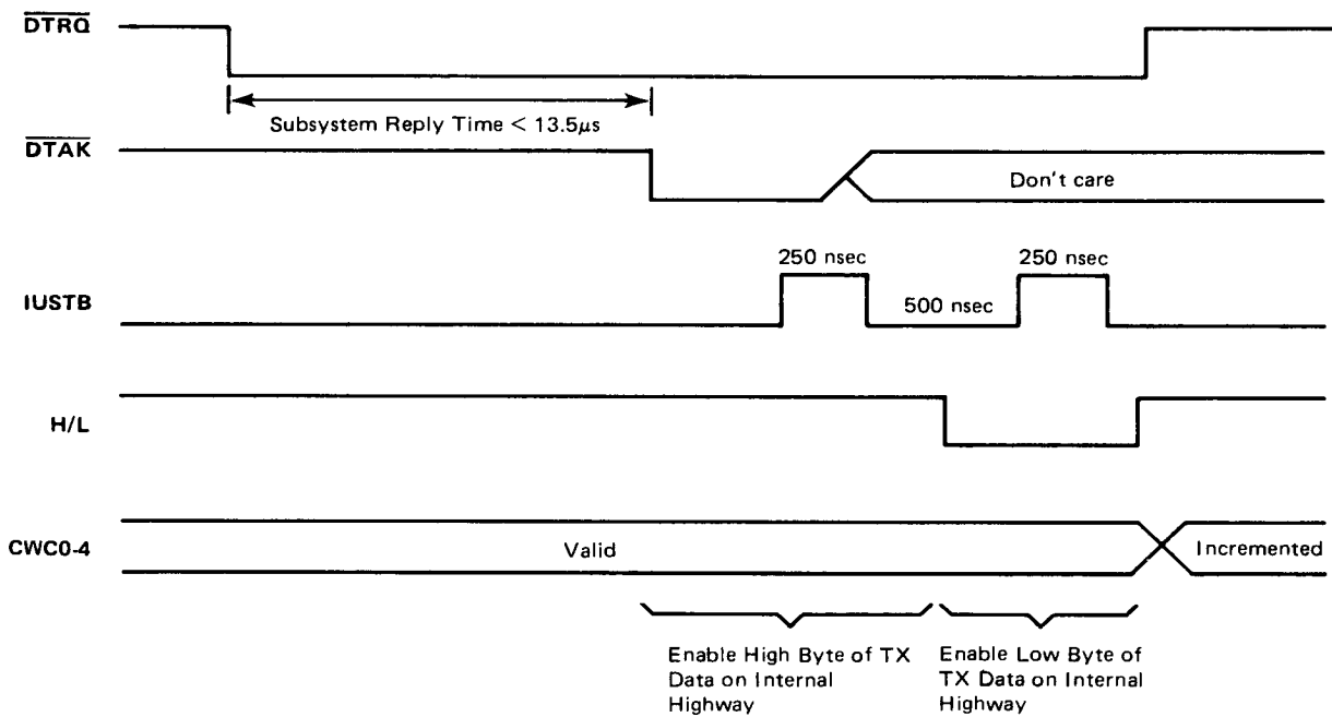
FIGURE 11. HANDSHAKING FOR Tx DATA TRANSFERS
