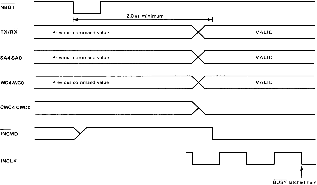
FIGURE 13. NEW COMMAND INITIALIZATION
