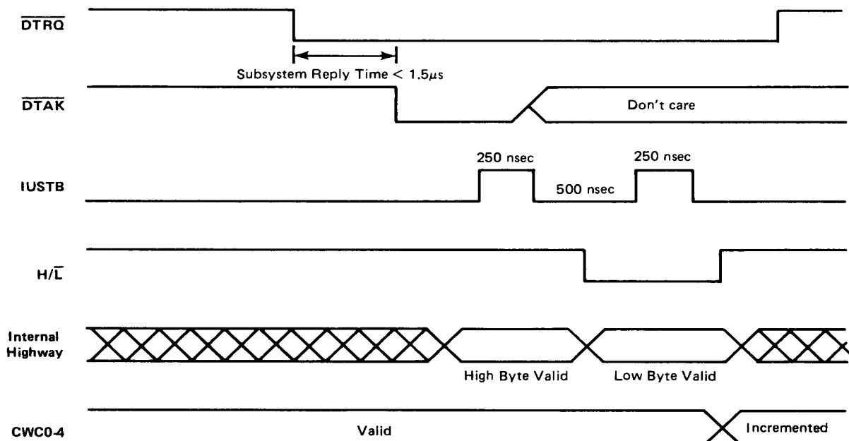
FIGURE 12. HANDSHAKING FOR Rx DATA TRANSFERS
