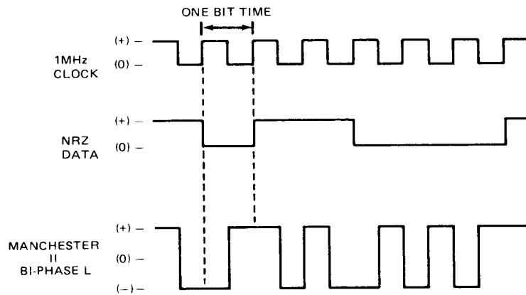
FIGURE 3. DATA ENCODING
