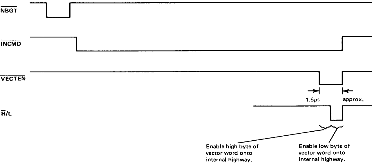
FIGURE 14. TRANSMIT VECTOR WORD COMMAND
