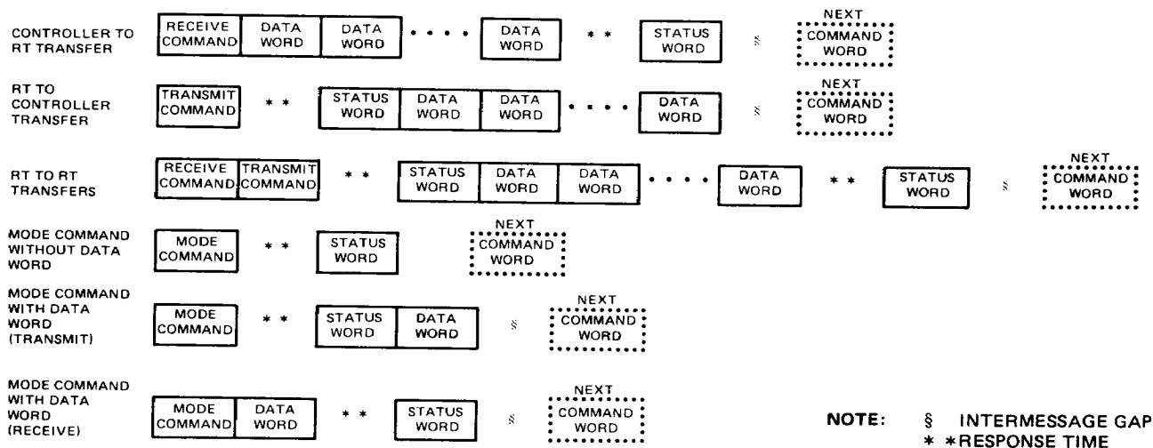
FIGURE 1. TYPICAL MESSAGE FORMATS
