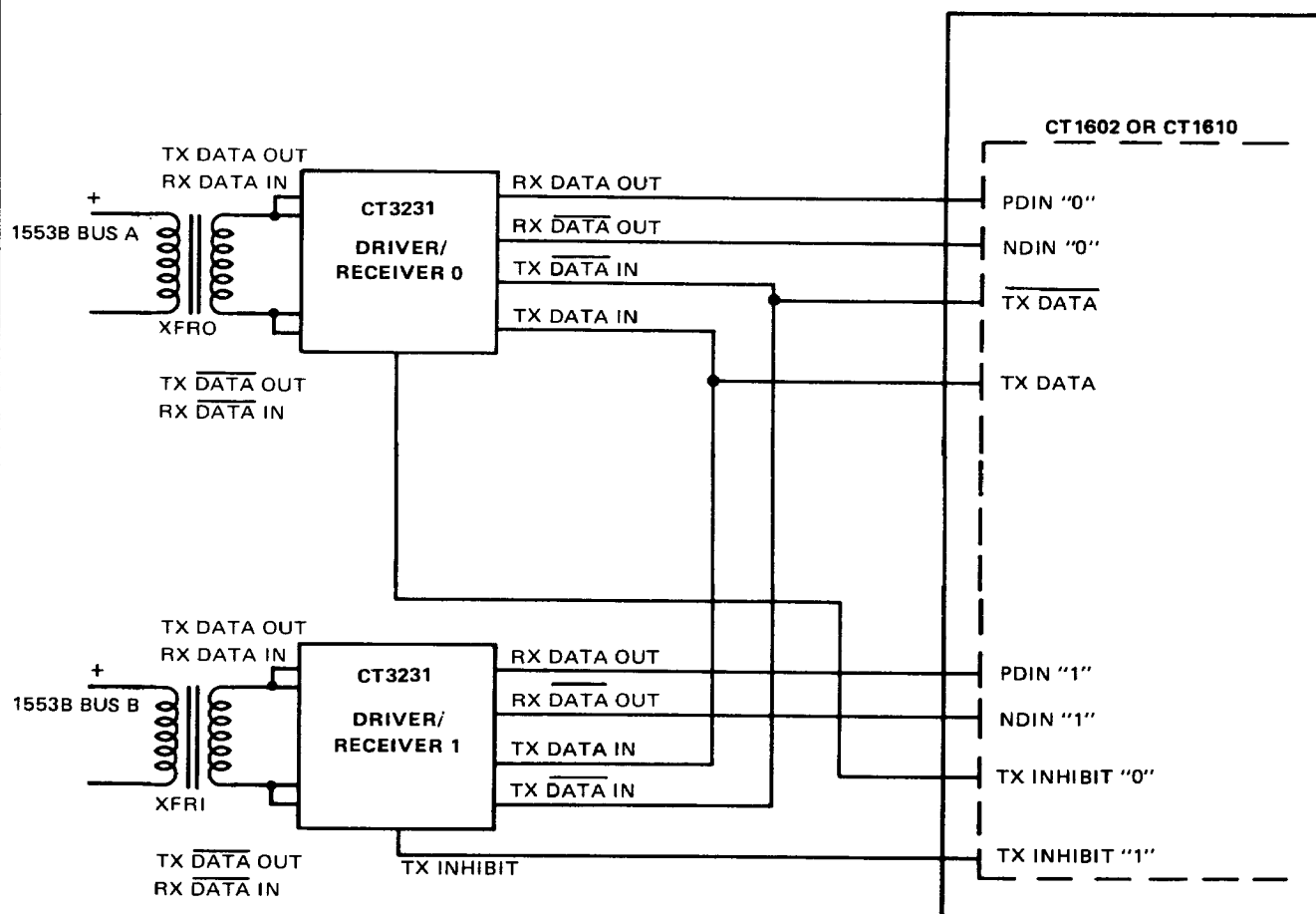
FIGURE 5. Example of an Interface between the CT1602 or CT1610 and Driver/Receiver
