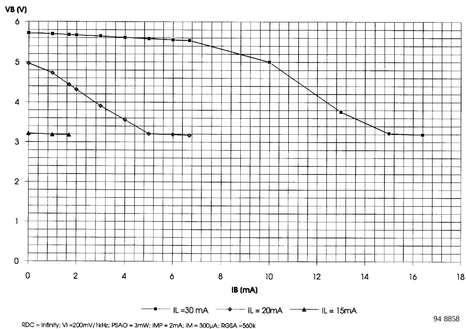
Figure 16. Typical load characteristic of V_B for a maximum ( RDC = \text{infinity} ) DC-characteristic and 3-mW loudspeaker output
