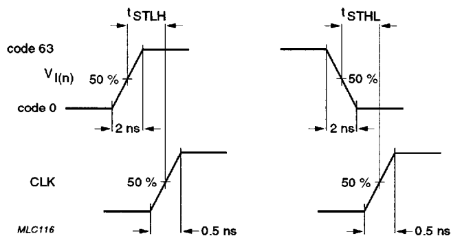
Fig.4 Analog input settling-time diagram.
