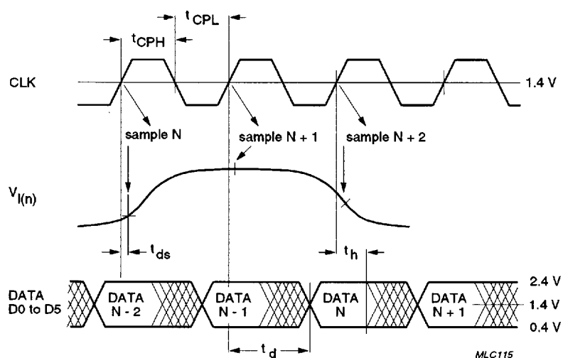
Fig.3 Timing diagram for data output.
