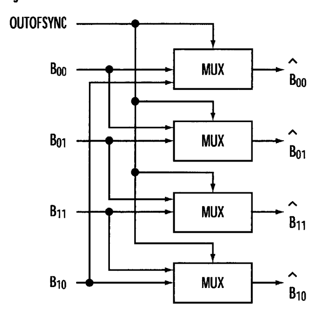
Figure 20. Branch Metric Rotation
