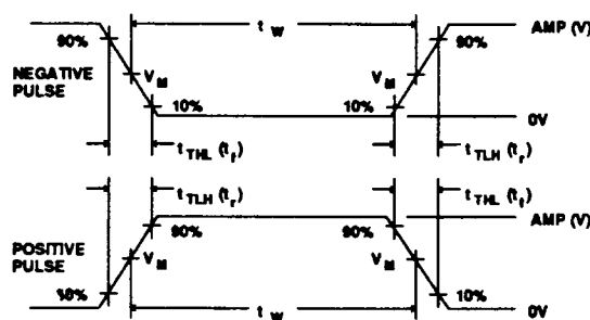
V_M = 1.5V Input Pulse Definition
