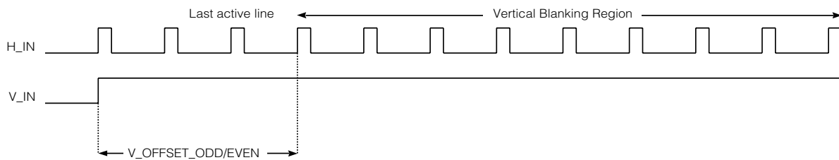
Fig. 3 Vertical Offset Definition
