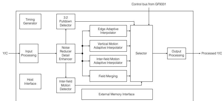
BLOCK DIAGRAM
