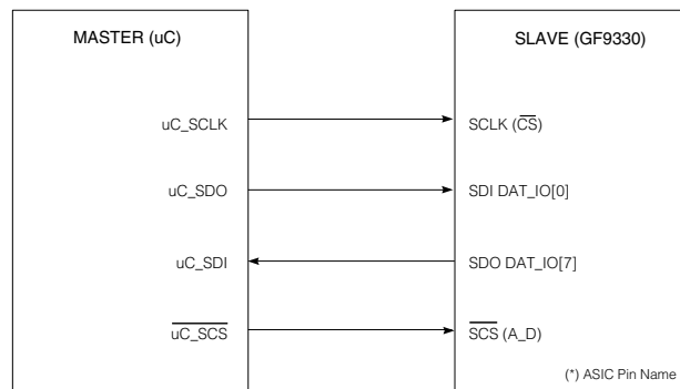
Fig. 4 Host Interface Serial Mode
