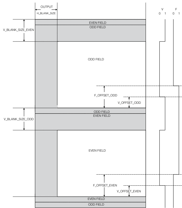
Fig. 2 Generic Input Format Definition
