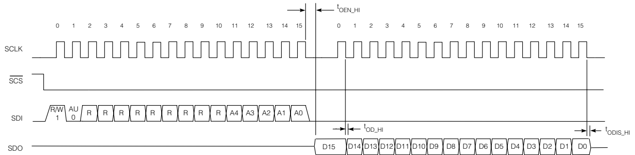
Fig. 8 Read Cycle
