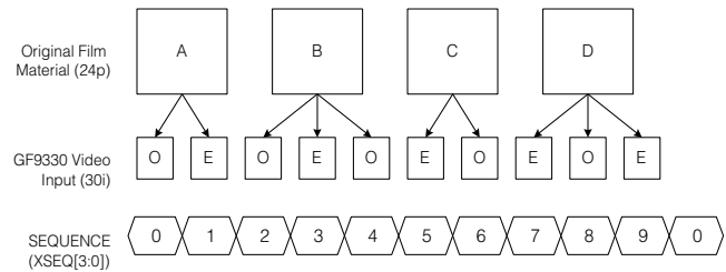
Fig.11 Sequence Detection Input Signals
