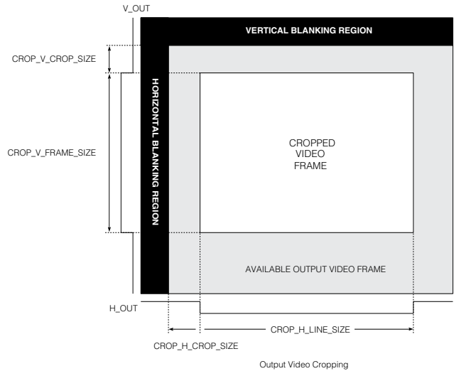
Fig. 12 Output Video Cropping
