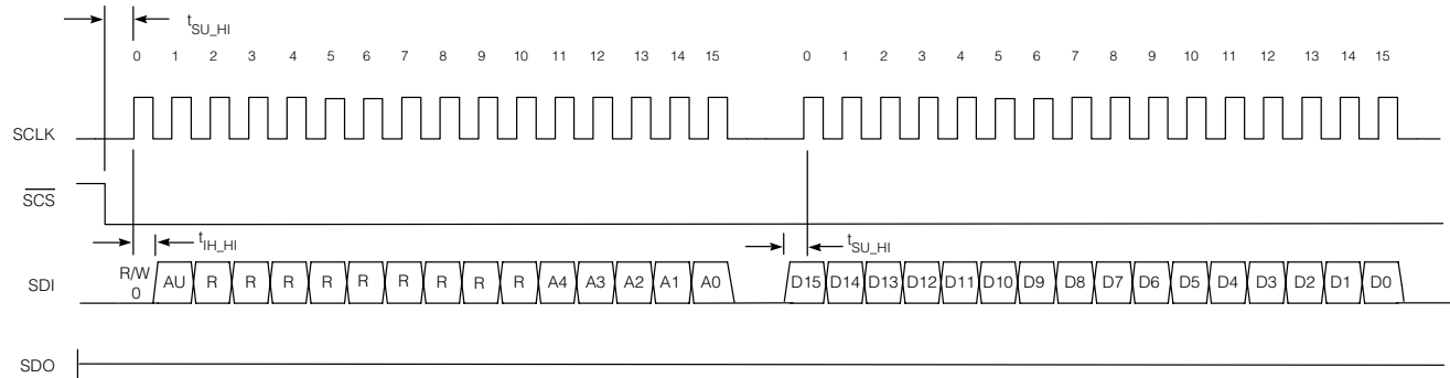
Fig. 7 Write Cycle
