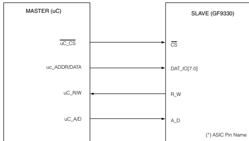
Fig. 9 Parallel Peripheral Interface
