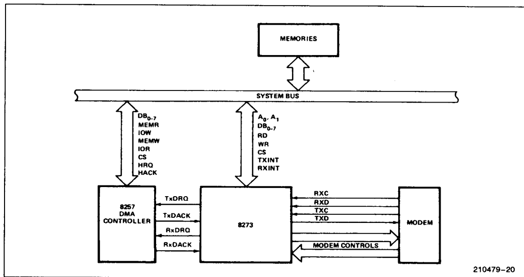
Figure 18. 8273 System Diagram
