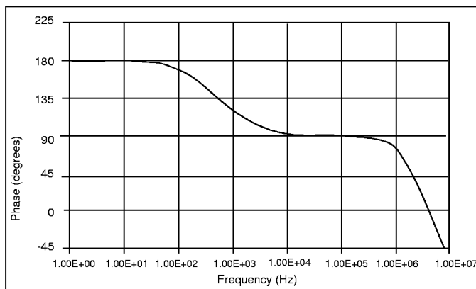
Figure 34: Error Amplifier Phase vs Frequency.
