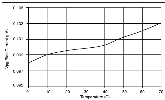
Figure 33: V_{\text{FB}} Bias Current vs Temperature.
