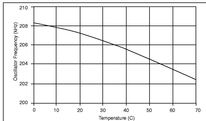
Figure 26: Oscillator Frequency vs Temperature. C_T = 330\text{pF} , R_T = 27\text{k}
