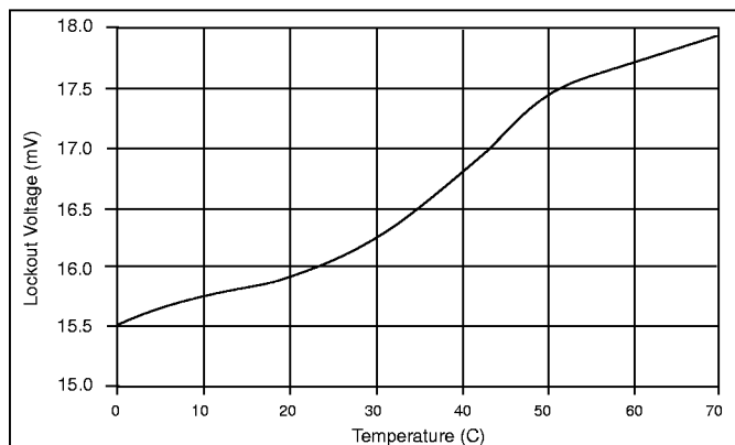
Figure 46: GATE Low Voltage (Lockout) vs Temperature.
