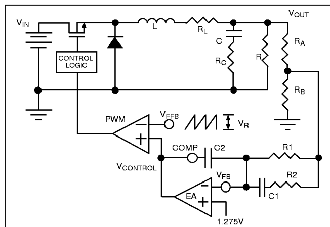
Figure 6: Voltage mode control equivalent circuit with two pole, one zero compensation network.
