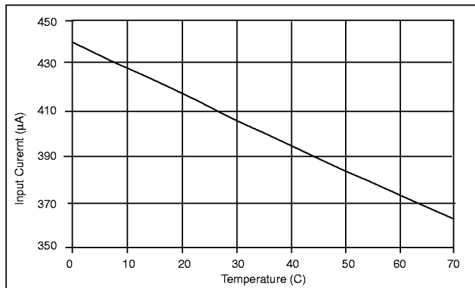
Figure 32: SYNC Input Current vs Temperature ( V_{\text{SYNC}} = 5\text{V} ).
