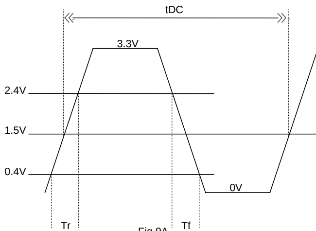
3.3V signals
