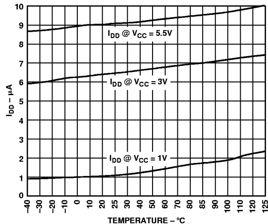
Figure 5. Supply Current vs. Temperature (ADM81_L/M)
