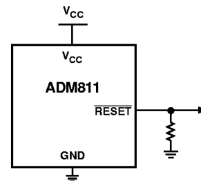
Figure 9. Ensuring a Valid \overline{\text{RESET}} Output Down to V_{CC} = 0 V
