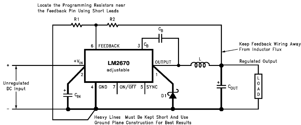
FIGURE 2. Basic circuit for adjustable output voltage applications
