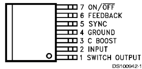
TO-263 Package Top View
