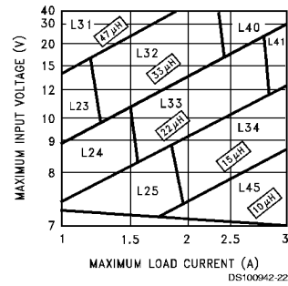
FIGURE 4. LM2670-5.0
