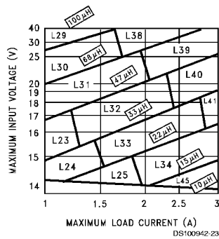
FIGURE 5. LM2670-12
