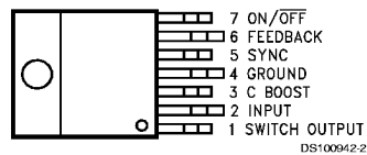
TO-220 Package Top View
