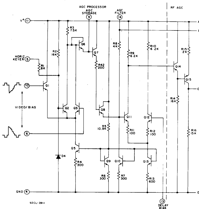
Fig.3 — Schematic diagram.
