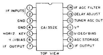
Fig.4 – Terminal assignment.
