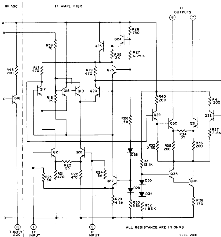
Fig.3 – Schematic diagram.
