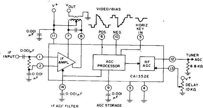
Fig. 1 — Block diagram.
