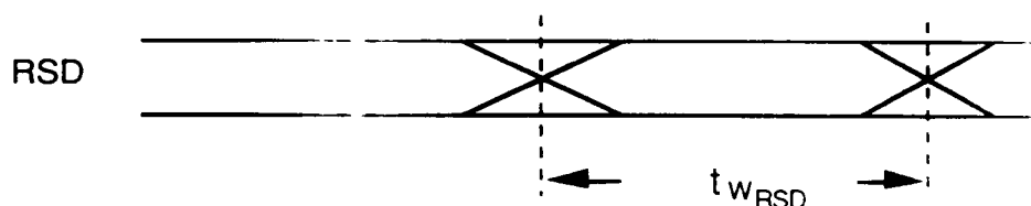
Fig. 31 STS-12 Receive Serial Data Input Timing
