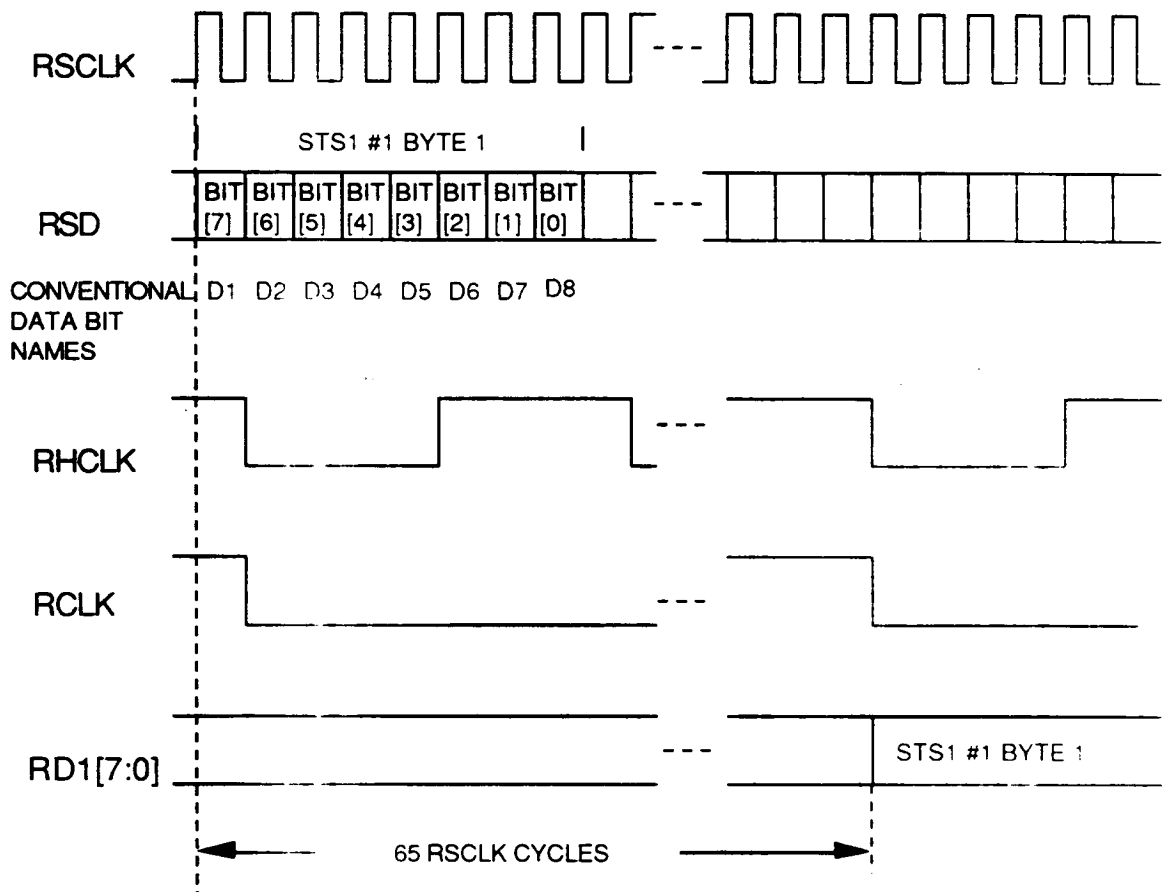
Fig. 1 Receive Input/Output Timing
