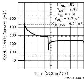
Short-Circuit Current
