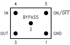
micro SMD, 5 Bump Package (BPA05)
