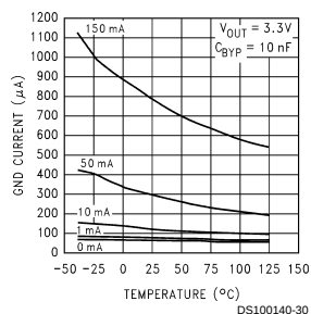
GND Pin Current vs Temperature
