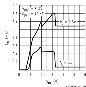
Input Current vs Pin
