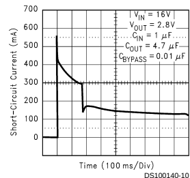
Short-Circuit Current
