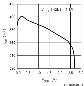
Short Circuit Current vs Output Voltage
