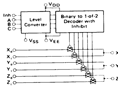
Figure 12 HD14053B Multiplexers/De-Multiplexers
