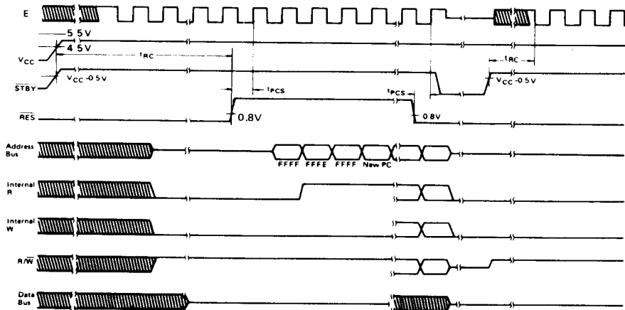
Figure 9 Reset Timing
