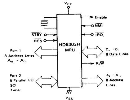
Figure 14 HD6303R MPU Non Multiplexed Mode
