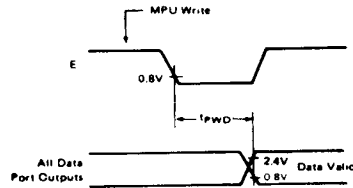
Note) Port 2: Except P 31 Figure 4 Port Data Delay Times (MPU Write)
