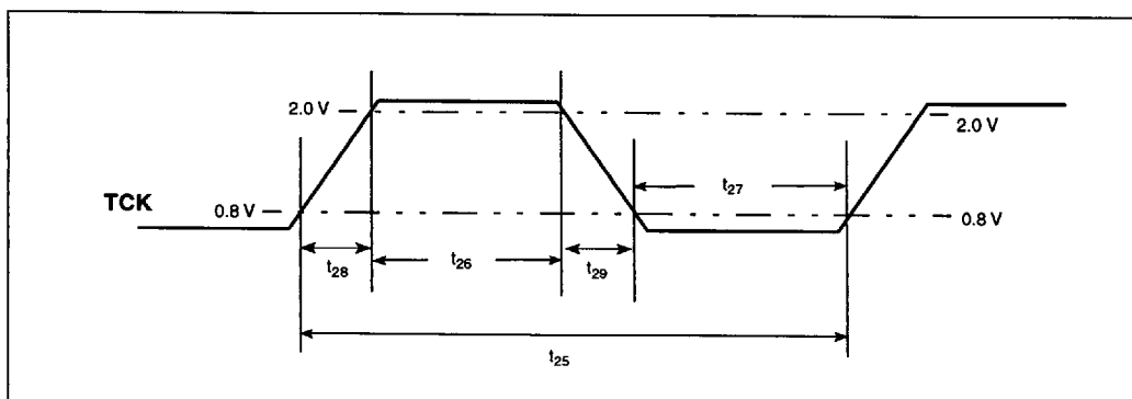
Figure 10. TCK Waveform
