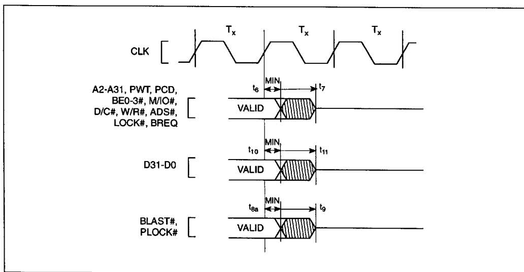
Figure 9. Maximum Float Delay Timing
