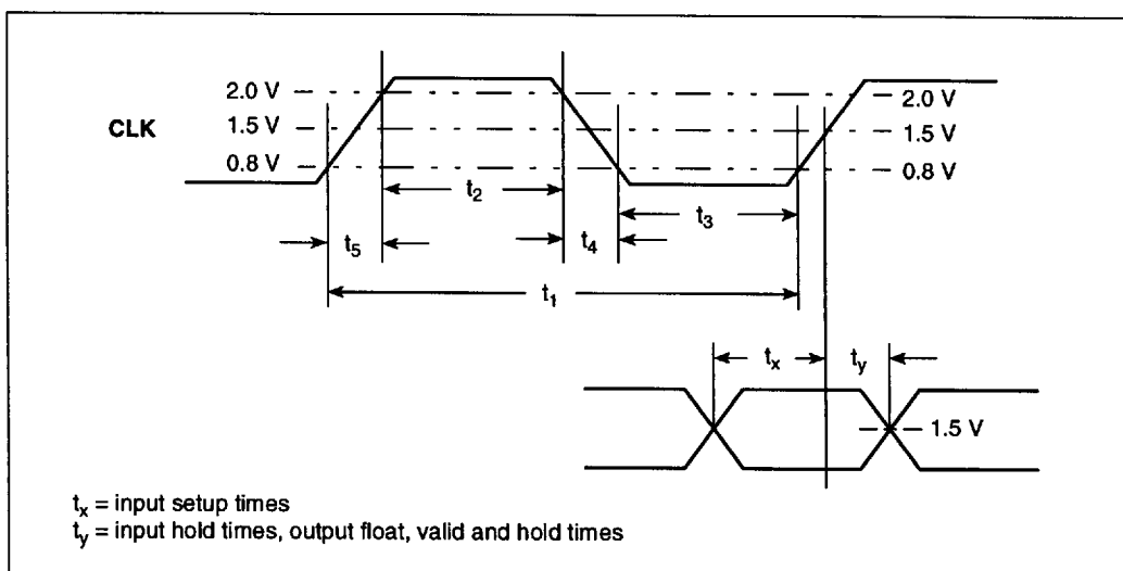
Figure 5. CLK Waveform
