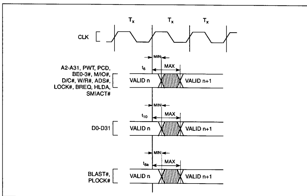
Figure 8. Output Valid Delay Timing
