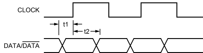
Figure 1. Data Timing Diagram
