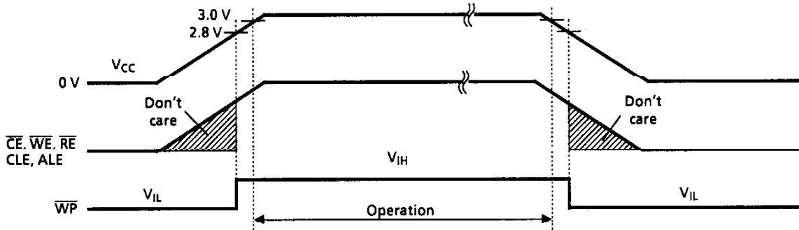
Figure 21. Power-on/off Sequence
