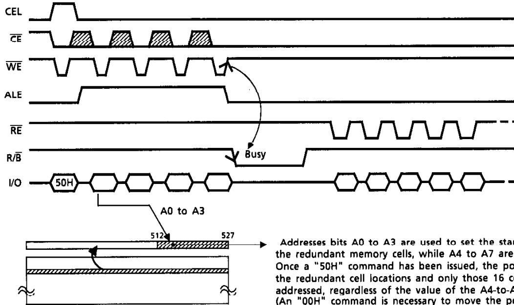
Figure 5. Read mode (3) operation
