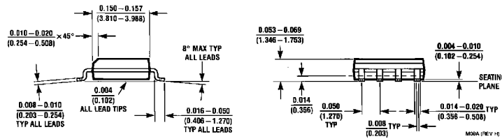
Molded Package SO (M) Order Number LM6365M NS Package Number M08A
