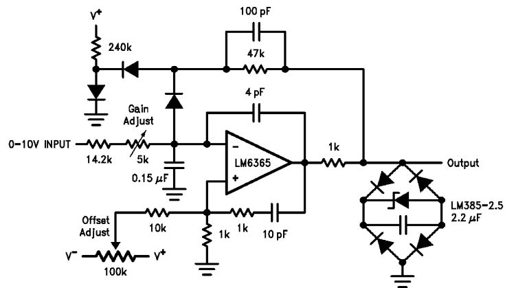
1 MHz Voltage-to-Frequency Converter ( f_{OUT} = 1 \text{ MHz} for V_{IN} = 10 \text{ V} )
