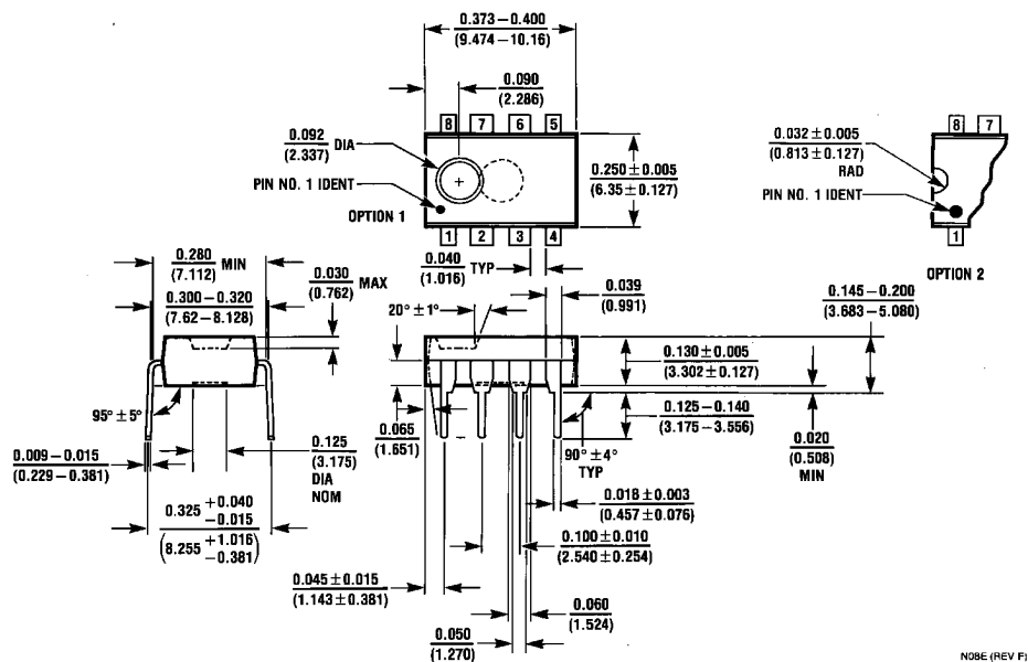
Molded Dual-In-Line Package (N) Order Number LM6265N or LM6365N NS Package Number N08E
