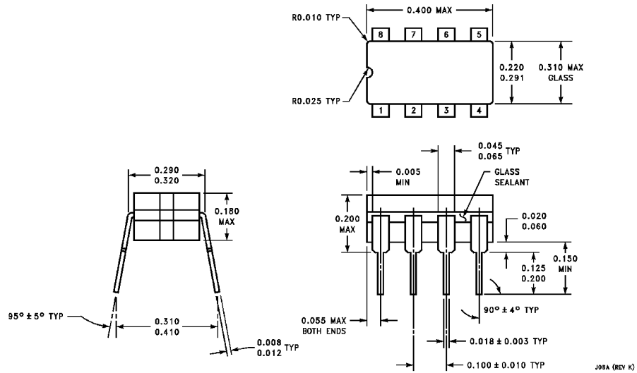
Ceramic Dual-In-Line Package (J) Order Number LM6165J/883 NS Package Number J08A
