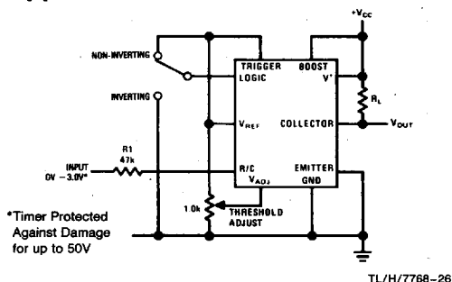
FIGURE 15. Comparator with 0V to 3V Threshold
