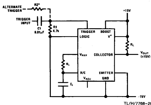
FIGURE 17. Operating Off Dual Supplies
