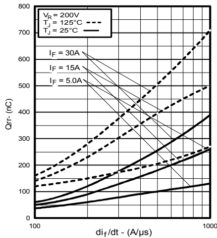
Fig. 7 - Typical Stored Charge vs. di/dt
