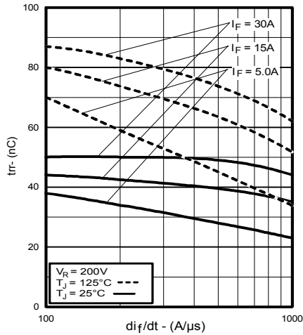
Fig. 5 - Typical Reverse Recovery vs. di/dt
