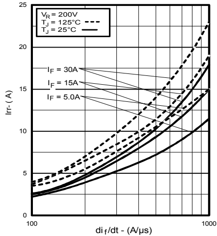
Fig. 6 - Typical Recovery Current vs. di/dt
