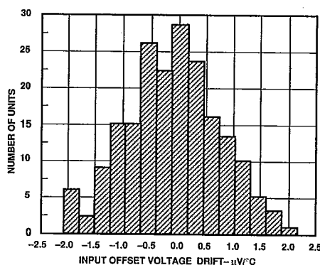
Typical Distribution of Average Input Offset
