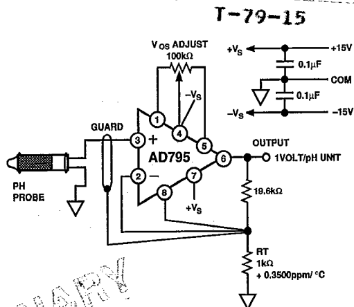
Figure 12. A pH Probe Amplifier
