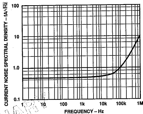
Figure 2. Current Noise Spectral Density
