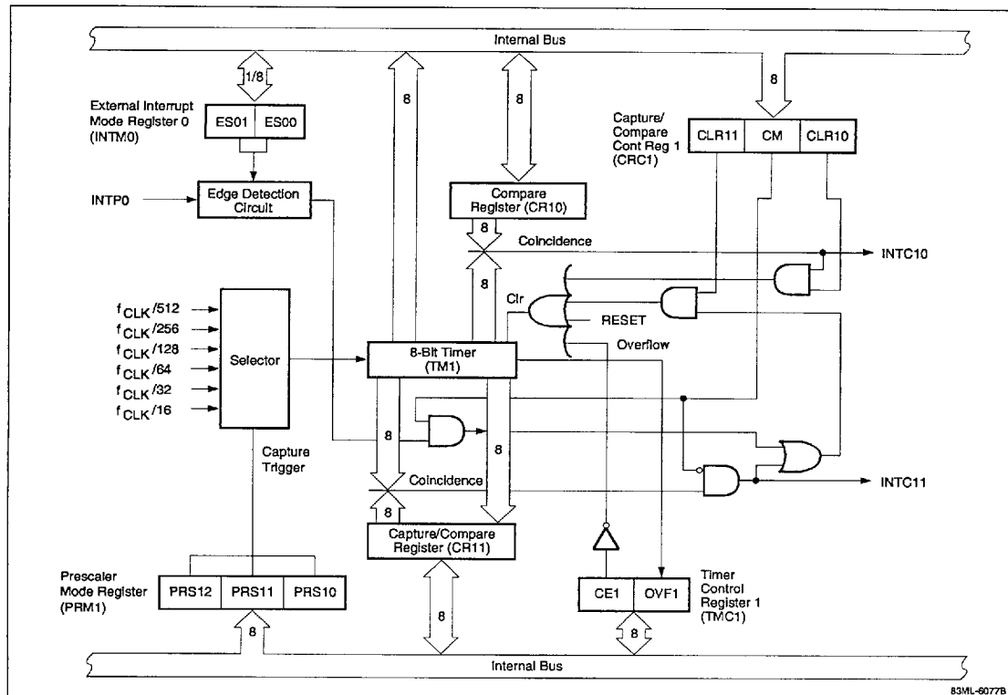
Figure 8. 8-Bit Timer/Counter 1
