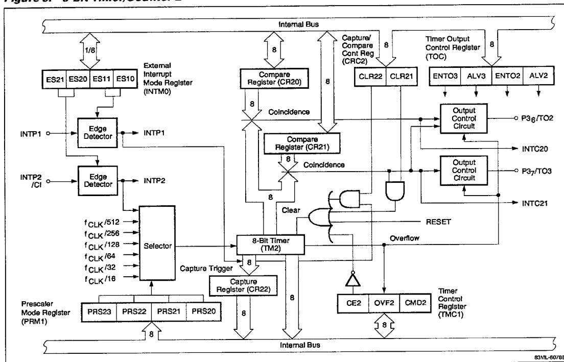
Figure 9. 8-Bit Timer/Counter 2
