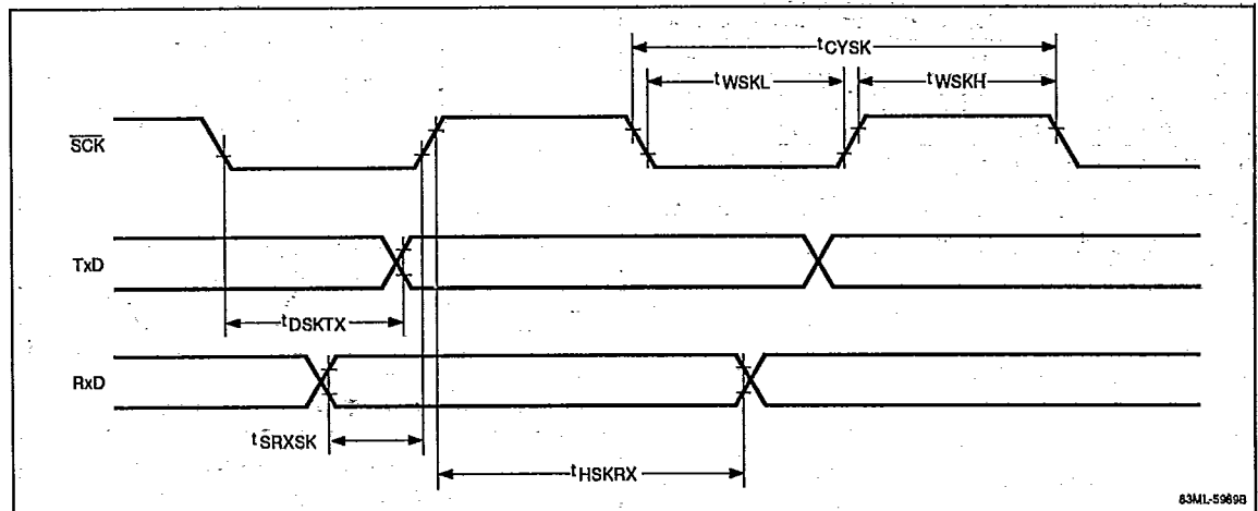
Figure 17. Asynchronous Mode Timing
