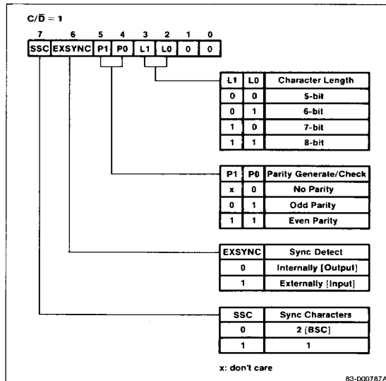
Figure 5. Mode byte for Setting Synchronous Mode
