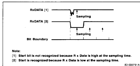
Figure 14. Asynchronous Receiver Example
