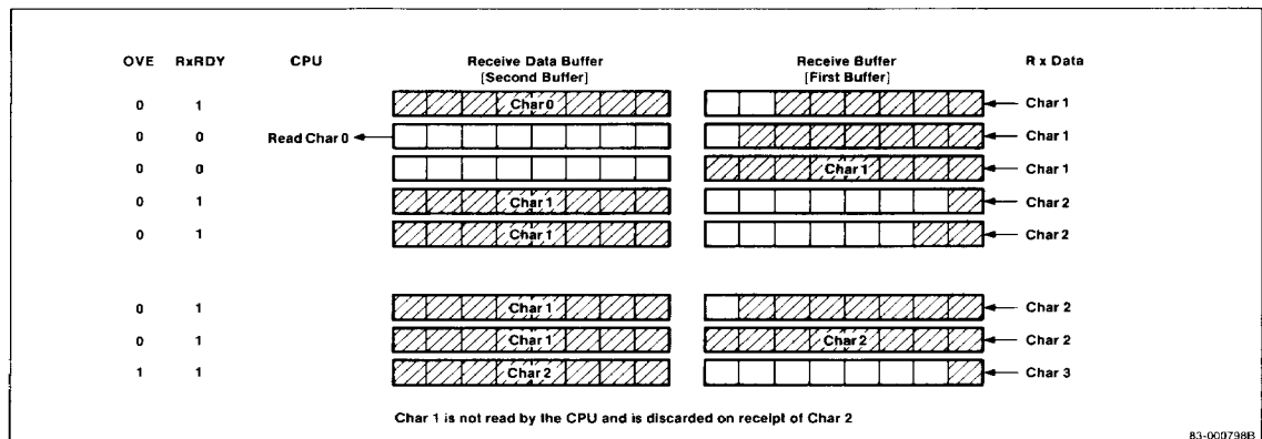
Figure 9. Overrun Error
