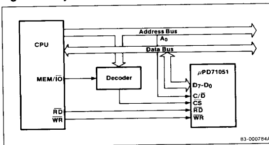
Figure 2. System Connection
