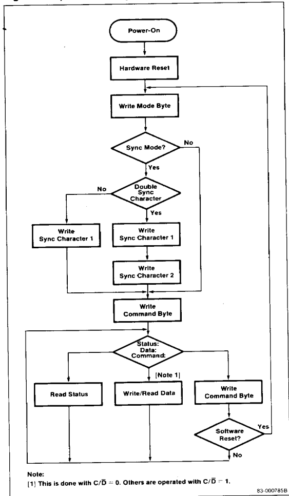
Figure 3. \mu PD71051 Operating Procedure
