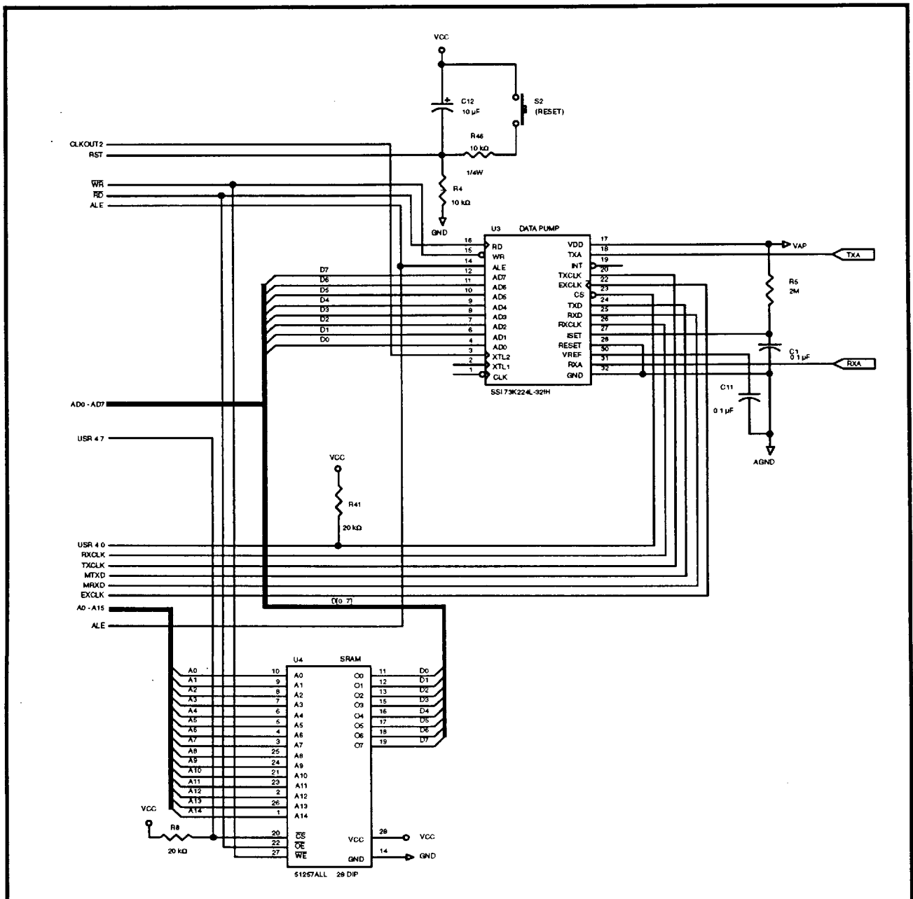
FIGURE 17B: Modem System Interconnect - Back End
