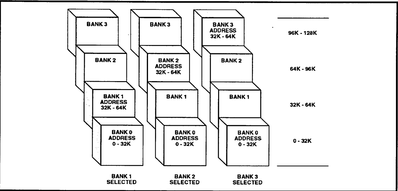
FIGURE 7: 128K of Bank-Selected Program Memory
