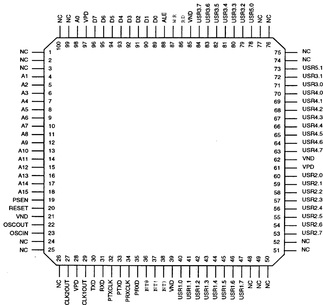
100-Lead TQFP
