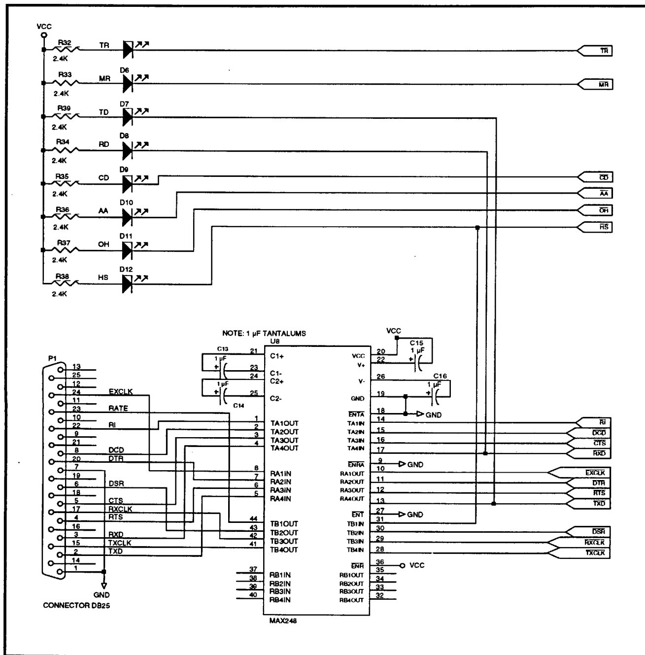
FIGURE 15: Display and User Interface
