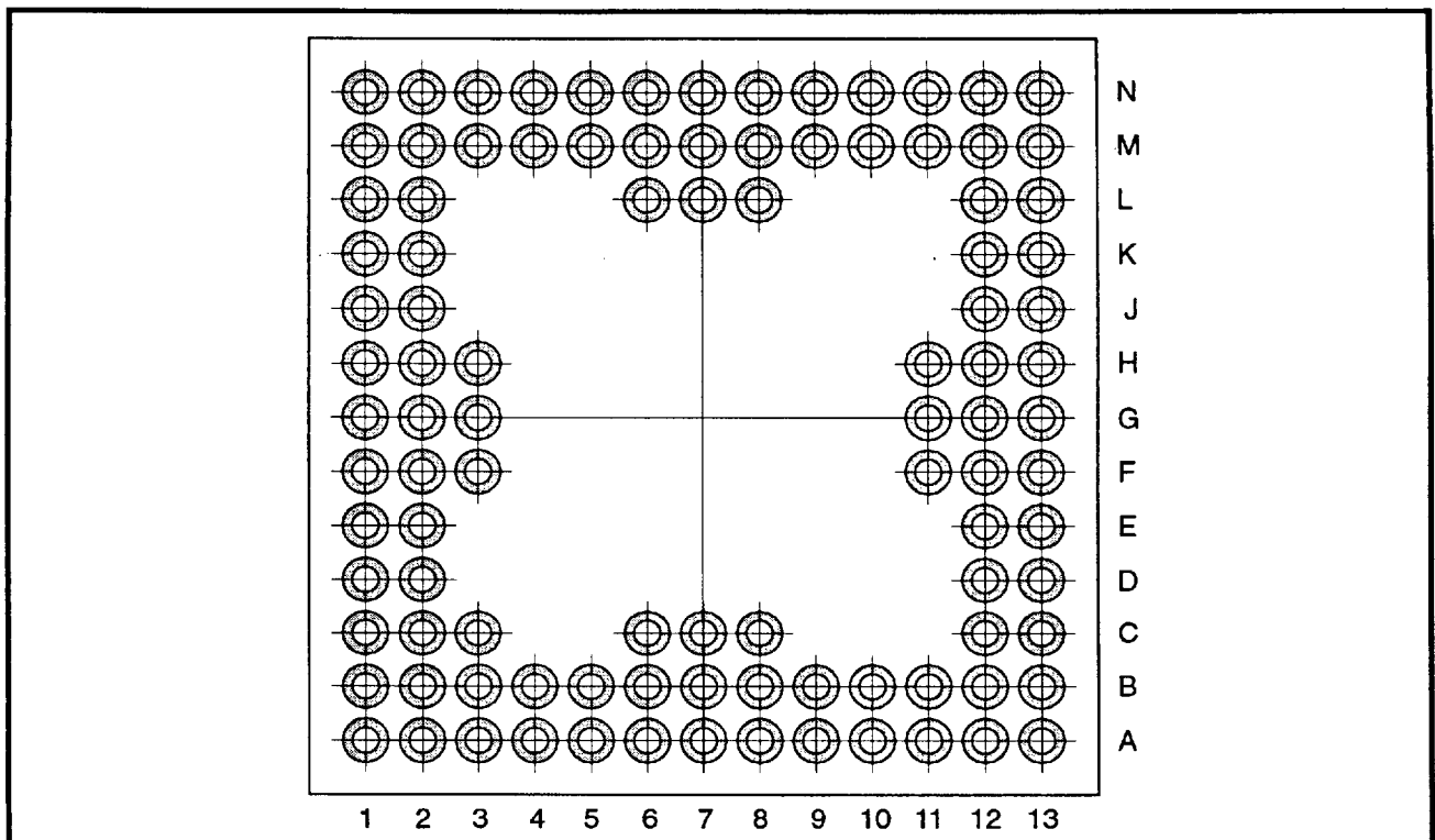
FIGURE 18: 100-Pin Grid Array (PGA) Package (Bottom View)
