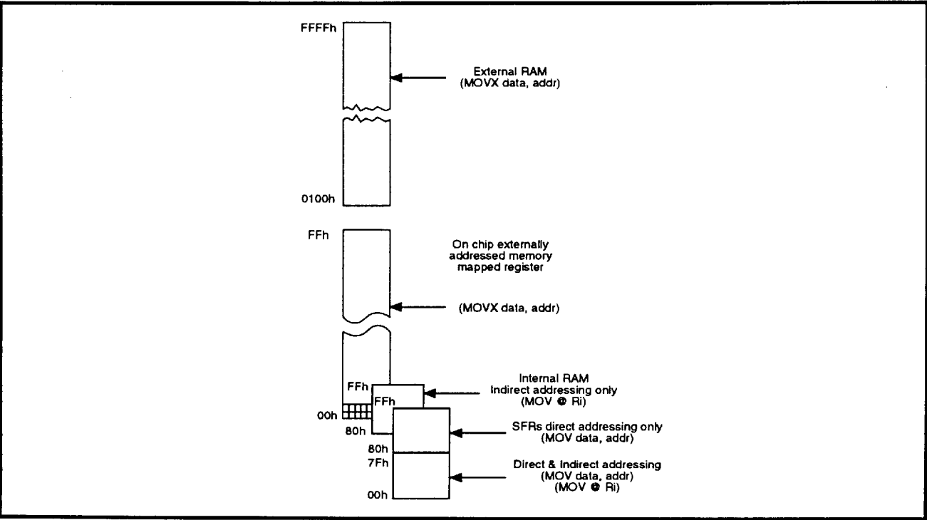
FIGURE 6: Memory Map
