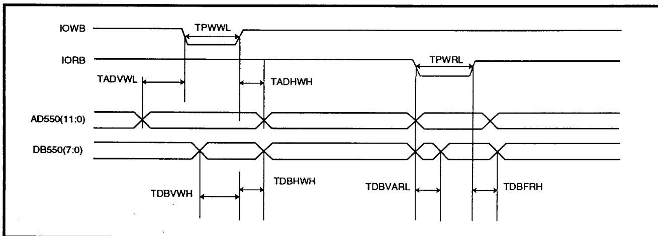
FIGURE 10: AC Timing
