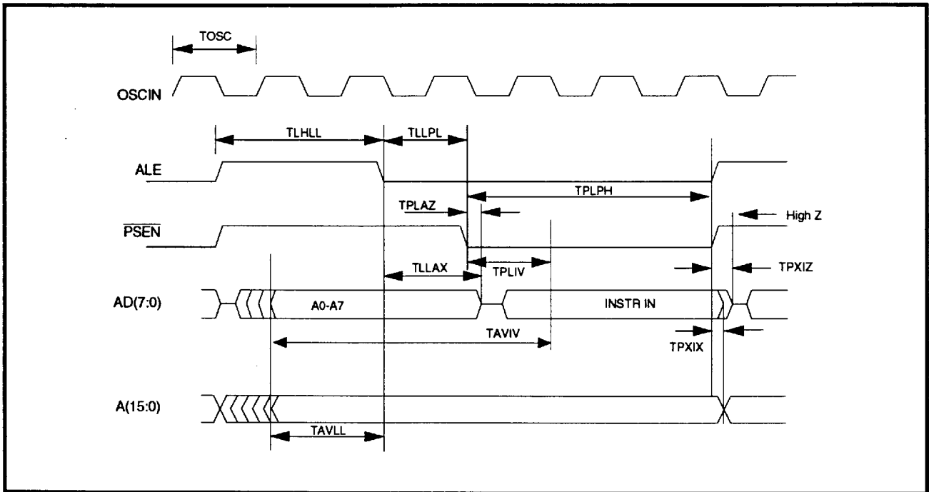
FIGURE 11: External Program Memory Read Cycle
