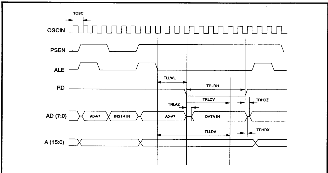
FIGURE 13: External Data Memory Read Cycle
