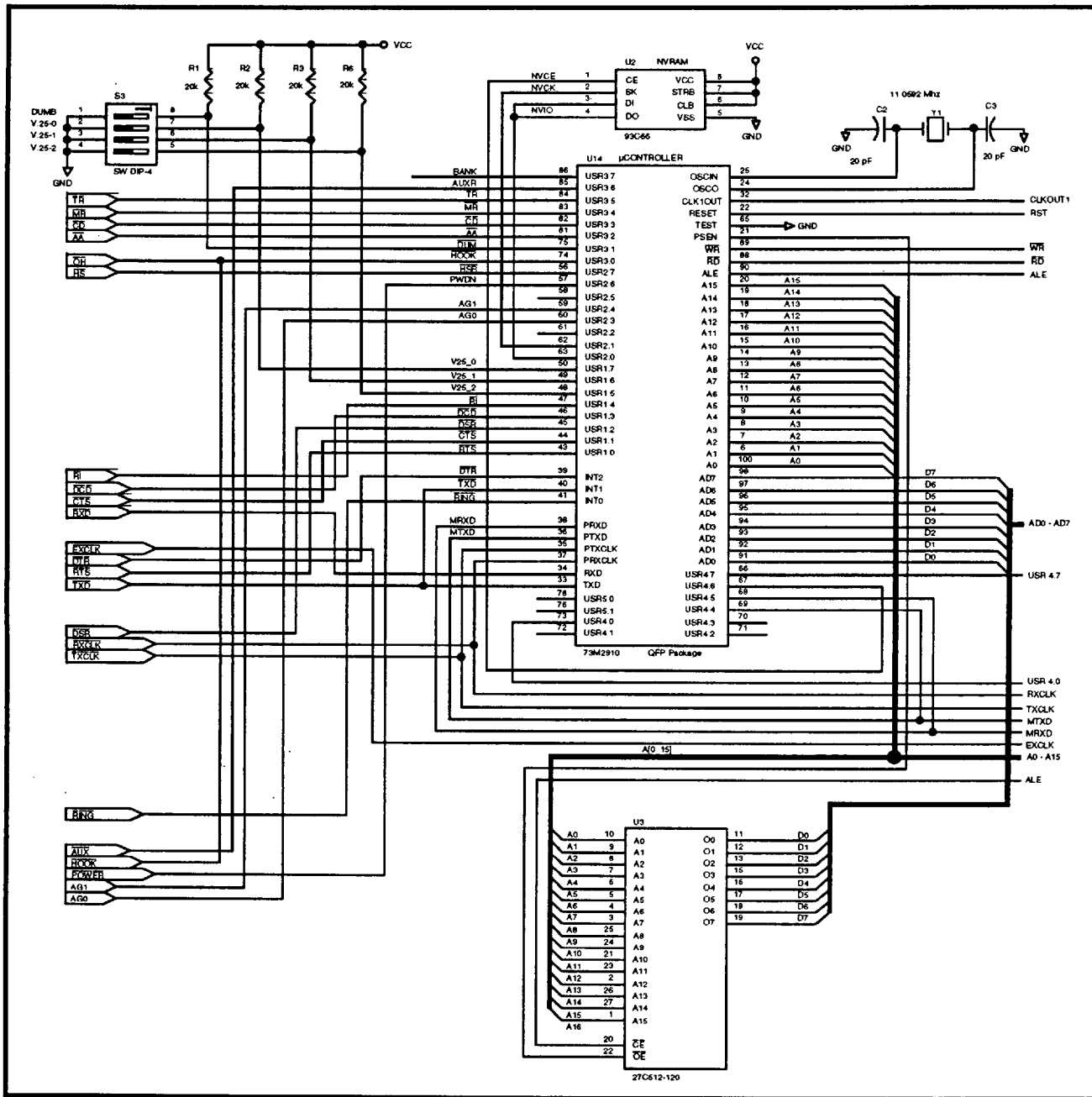
FIGURE 17A: Modem System Interconnect - Front End
