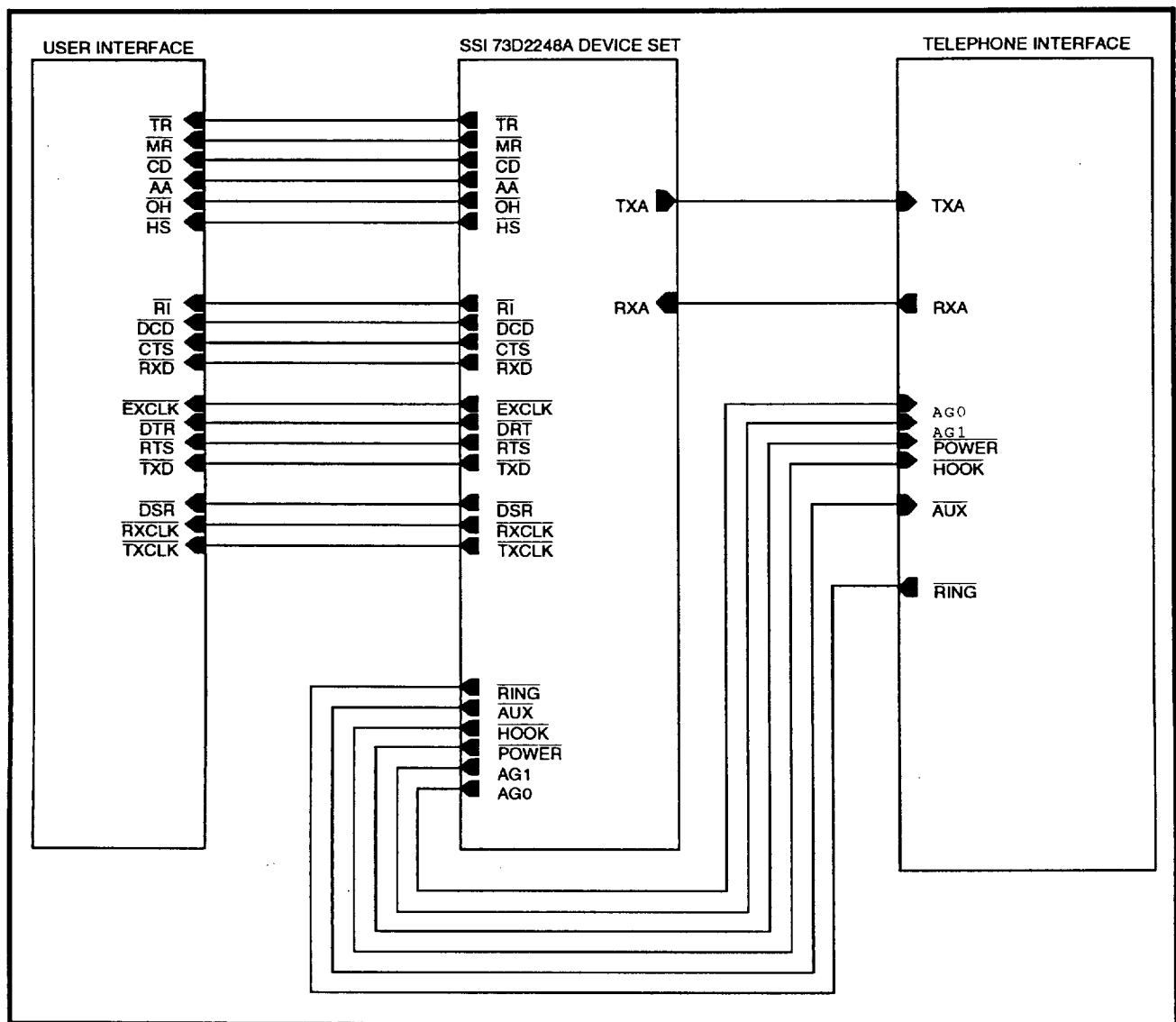
FIGURE 14: Modem Block Diagram
