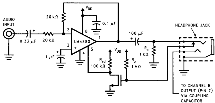
FIGURE 2. Automatic Shutdown Circuit
