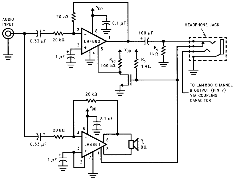
FIGURE 3. Automatic Switching Circuit
