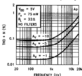
THD + N vs Frequency
