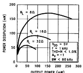
Power Dissipation vs Output Power
