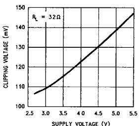
Clipping Voltage vs Supply Voltage
