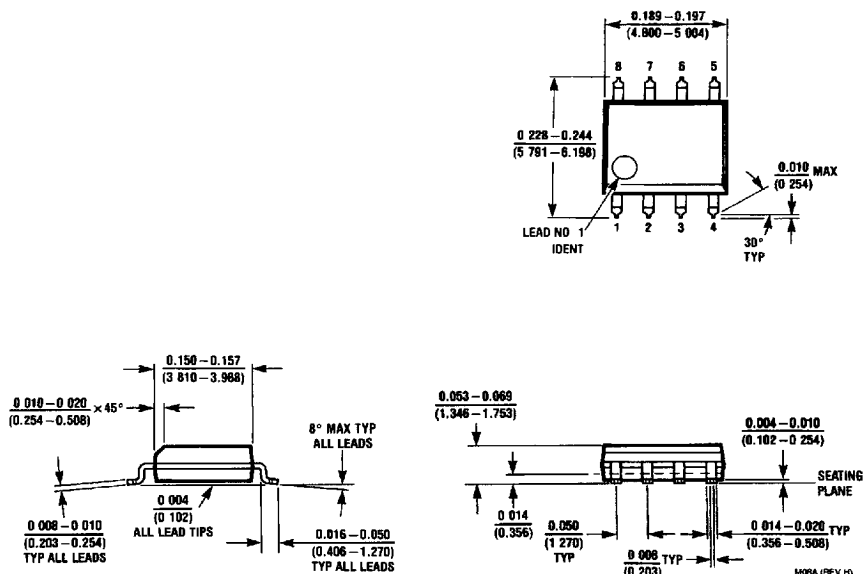
8-Lead (0.150" Wide) Molded Small Outline Package, JEDEC Order Number LM4880M NS Package Number M08A
