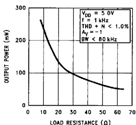
Output Power vs Load Resistance
