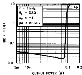
THD + N vs Output Power
