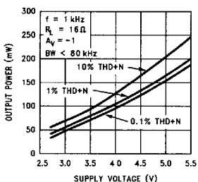
Output Power vs Supply Voltage
