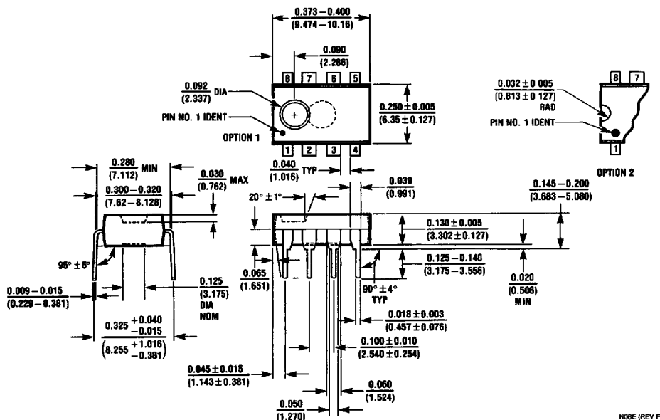
8-Lead (0.300" Wide) Molded Dual-In-Line Package Order Number LM4880N NS Package Number NO8E
