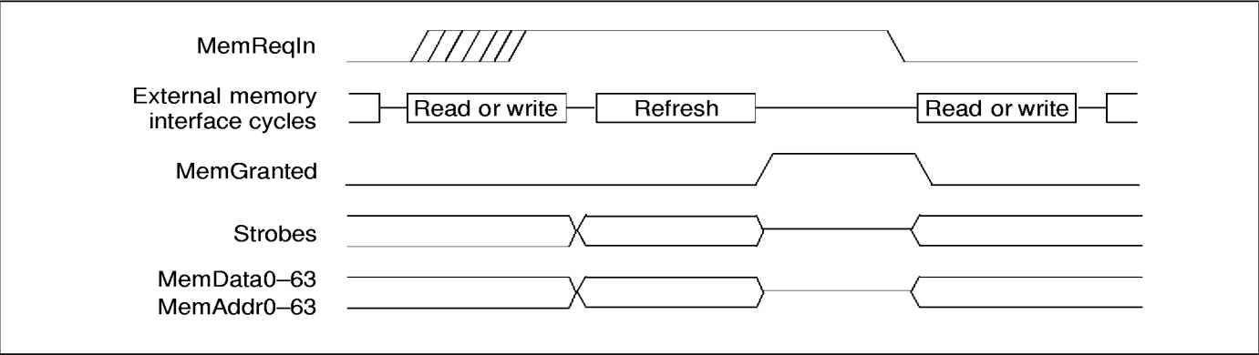
Figure 3.6 IMS T9000 operation of MemReqIn , MemGranted with external, refresh memory cycles
