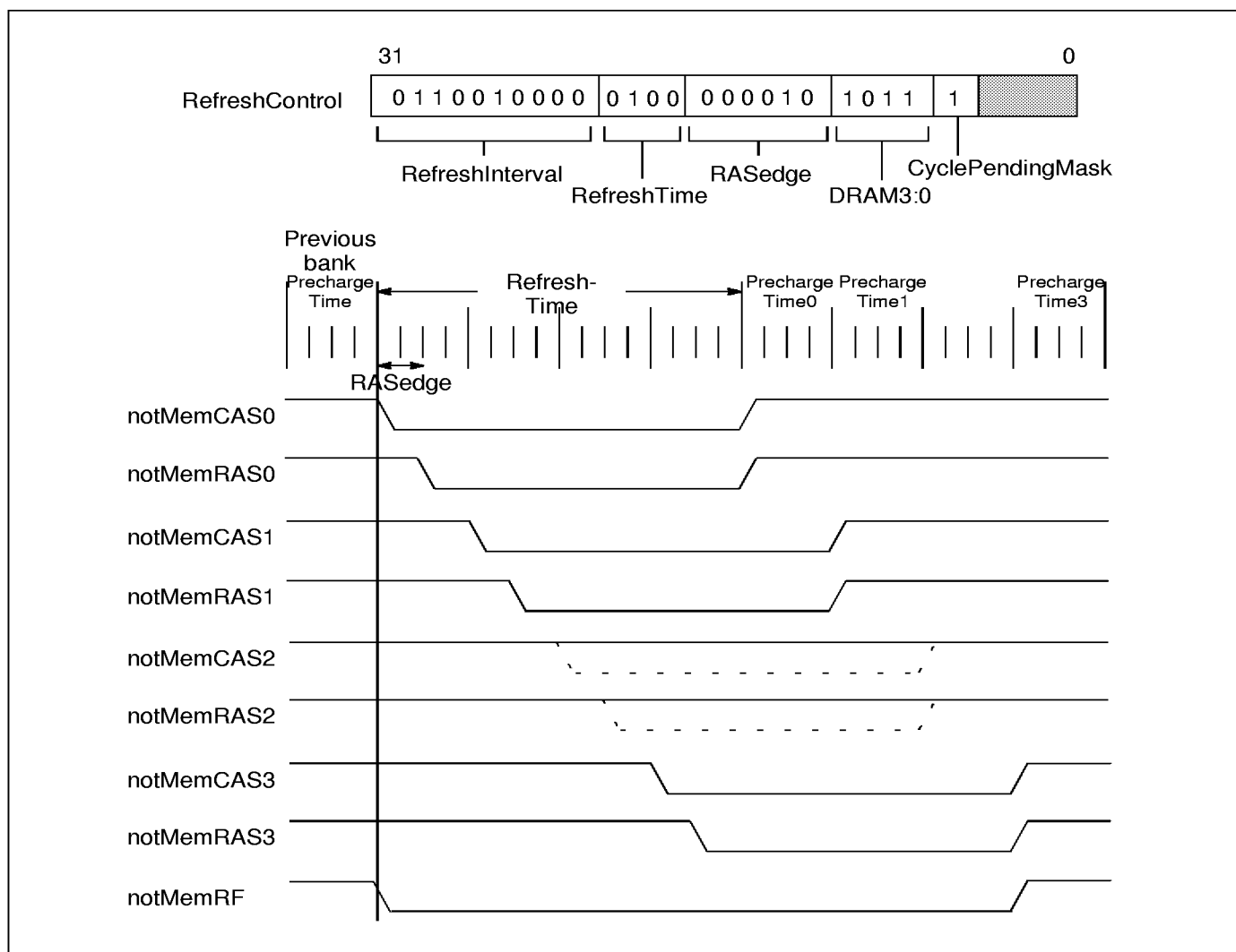
Figure 3.7 Programming of the refresh control register
