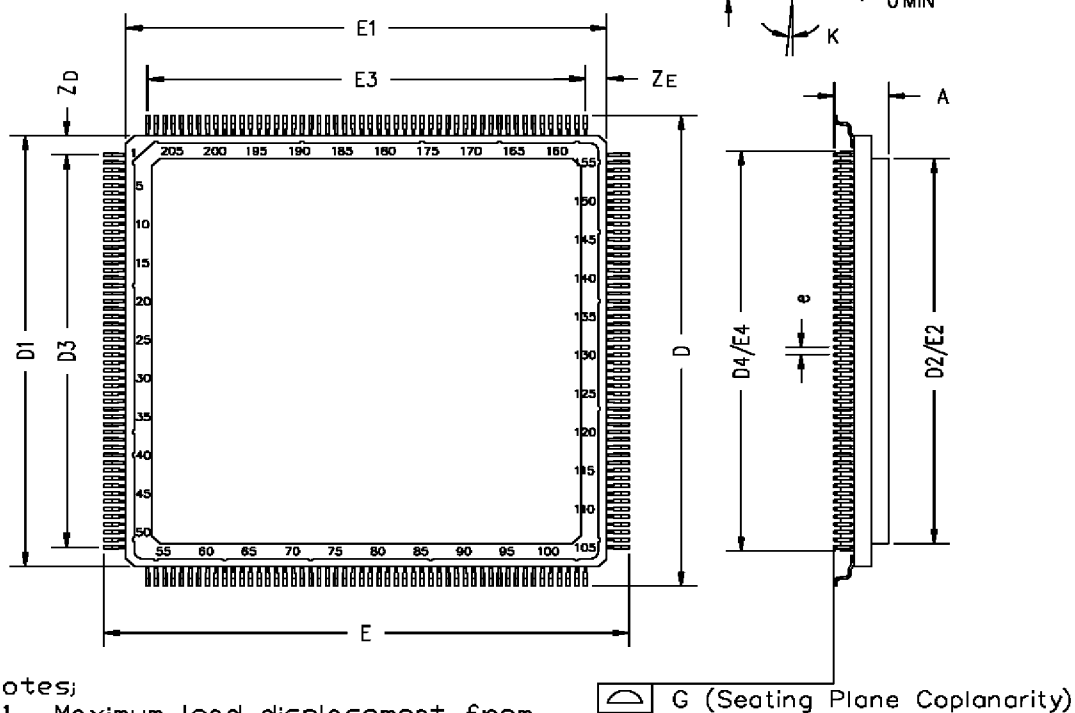
Figure 10.2 208 pin CLCC package dimensions
