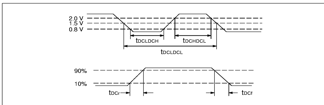
Figure 6.2 ClockIn timing
