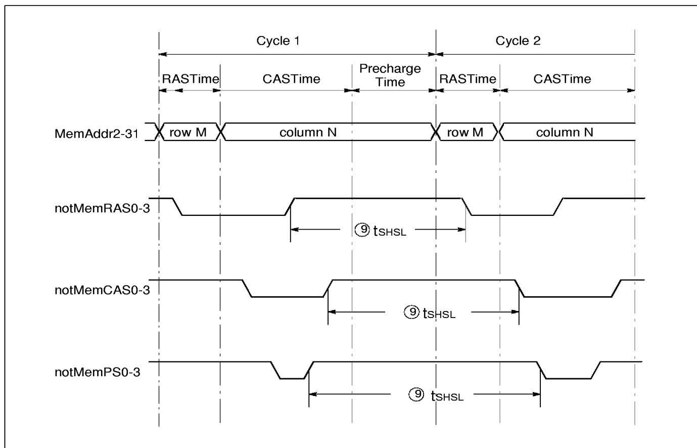
Figure 3.4 Cycle to cycle timing
