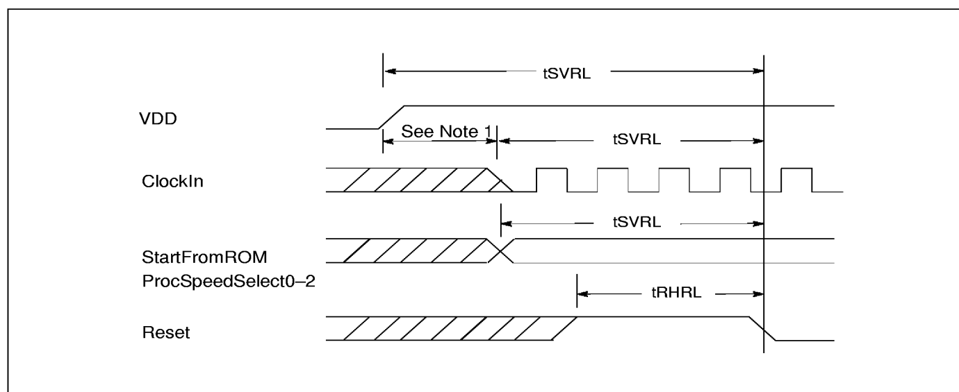
Figure 7.1 Timing for static signals
