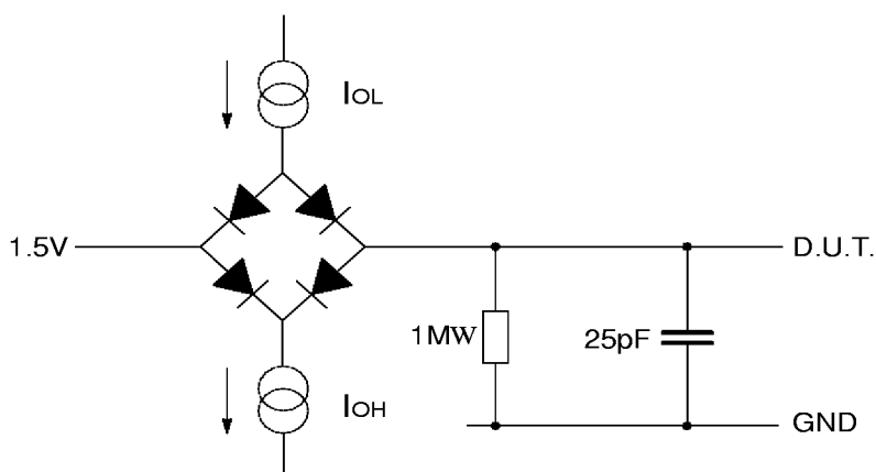
Figure 8.1 Load circuit for AC measurements
