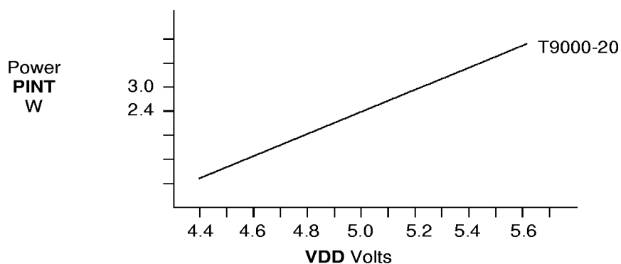
Figure 8.3 Internal power dissipation vs VDD
