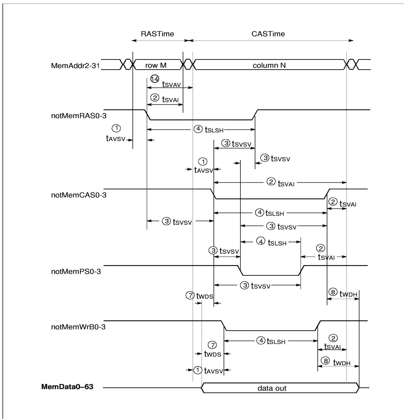
Figure 3.3 Write cycle timing
