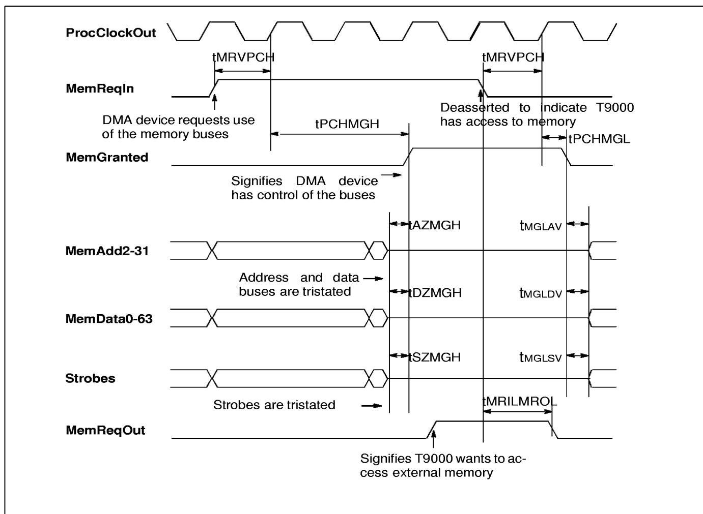
Figure 3.5 DMA
