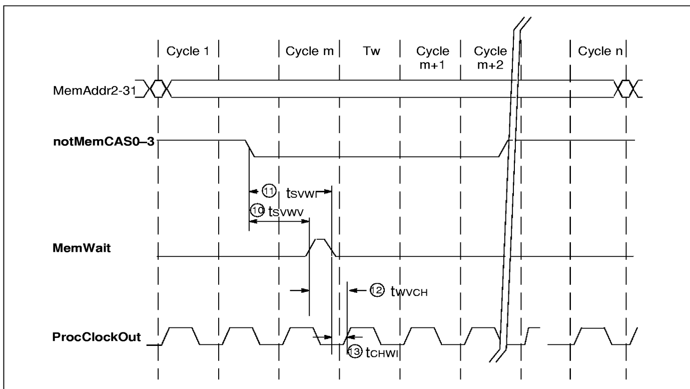
Figure 3.8 Memory wait timing
