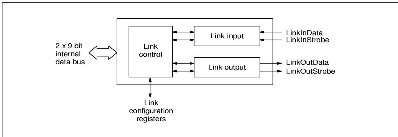
Figure 5.3 Link module
