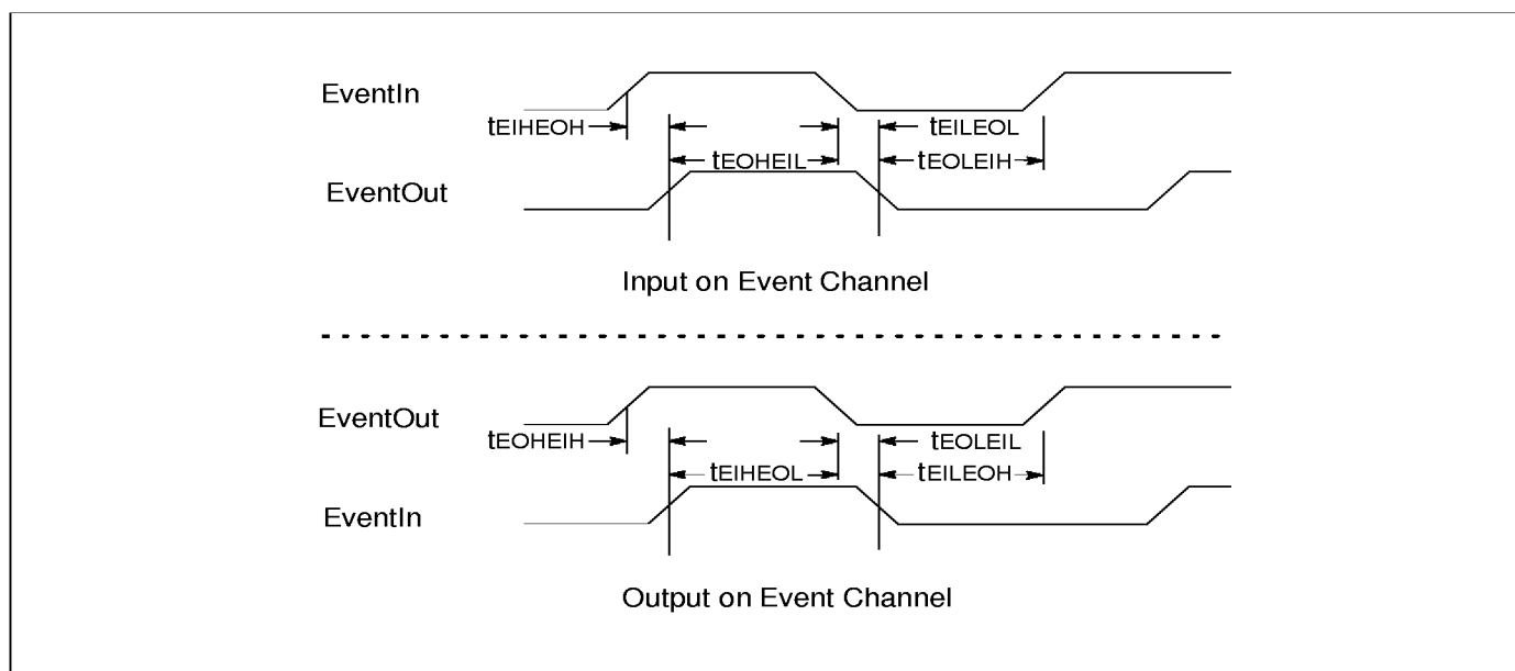
Figure 4.3 IMS T9000 event timing
