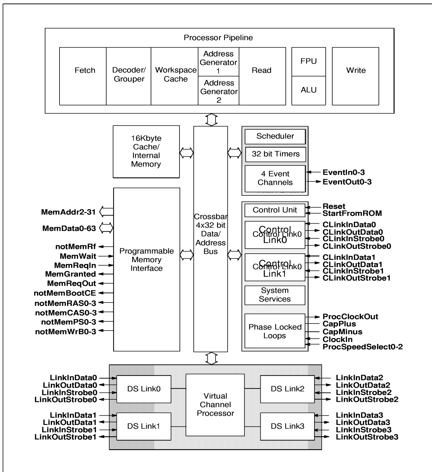
Figure 1.1 IMS T9000 block diagram
