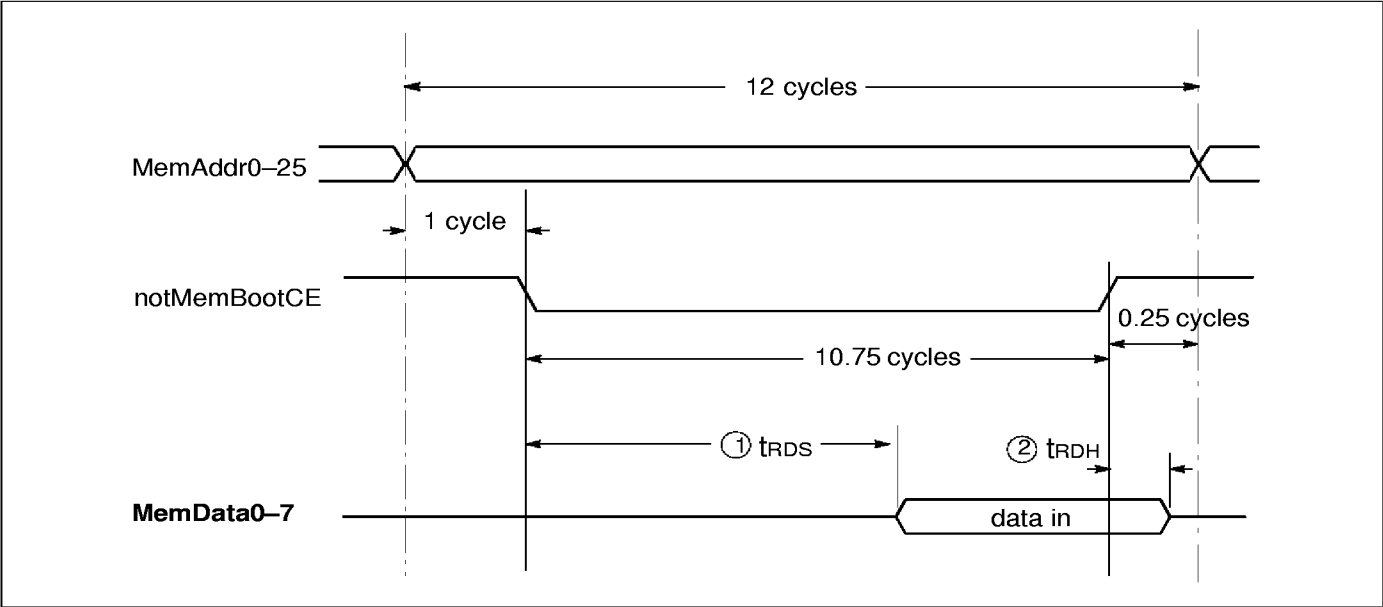
Figure 3.9 Boot cycle timing
