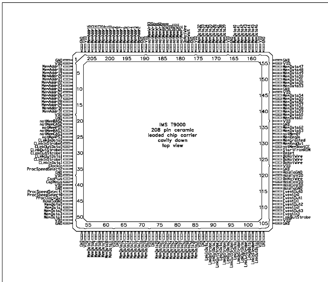
Figure 10.1 208 pin CLCC package pinout
