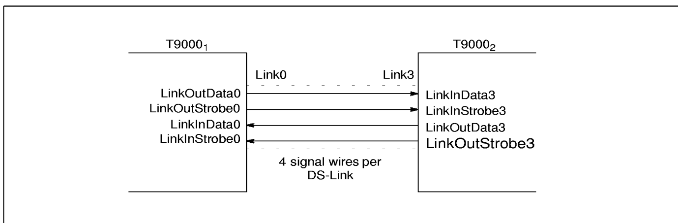
Figure 5.1 DS-Links
