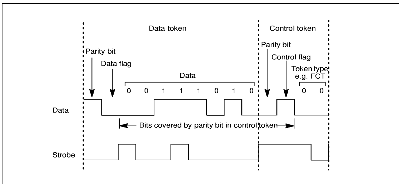
Figure 5.2 Link data and strobe formats
