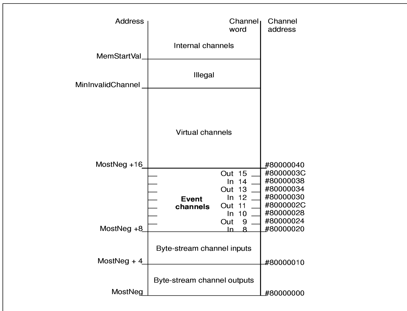
Figure 4.2 IMS T9000 channel address space
