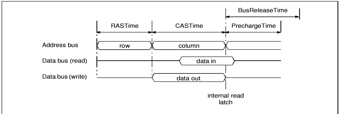
Figure 3.1 Generic memory cycle
