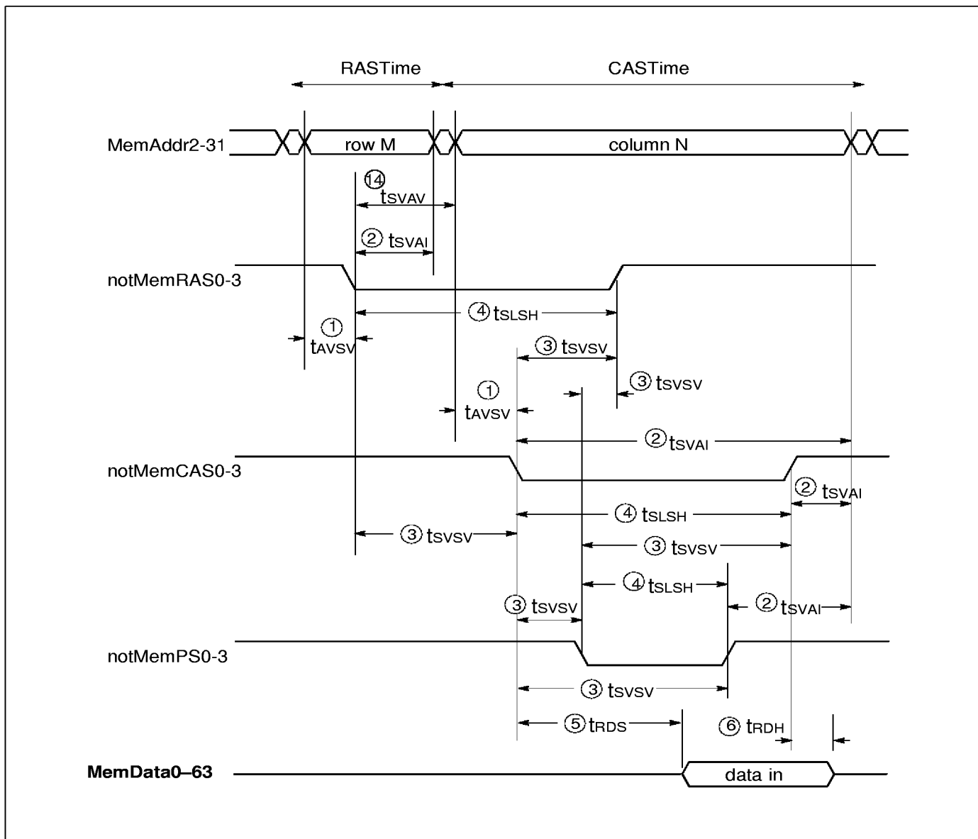
Figure 3.2 Read cycle timing
