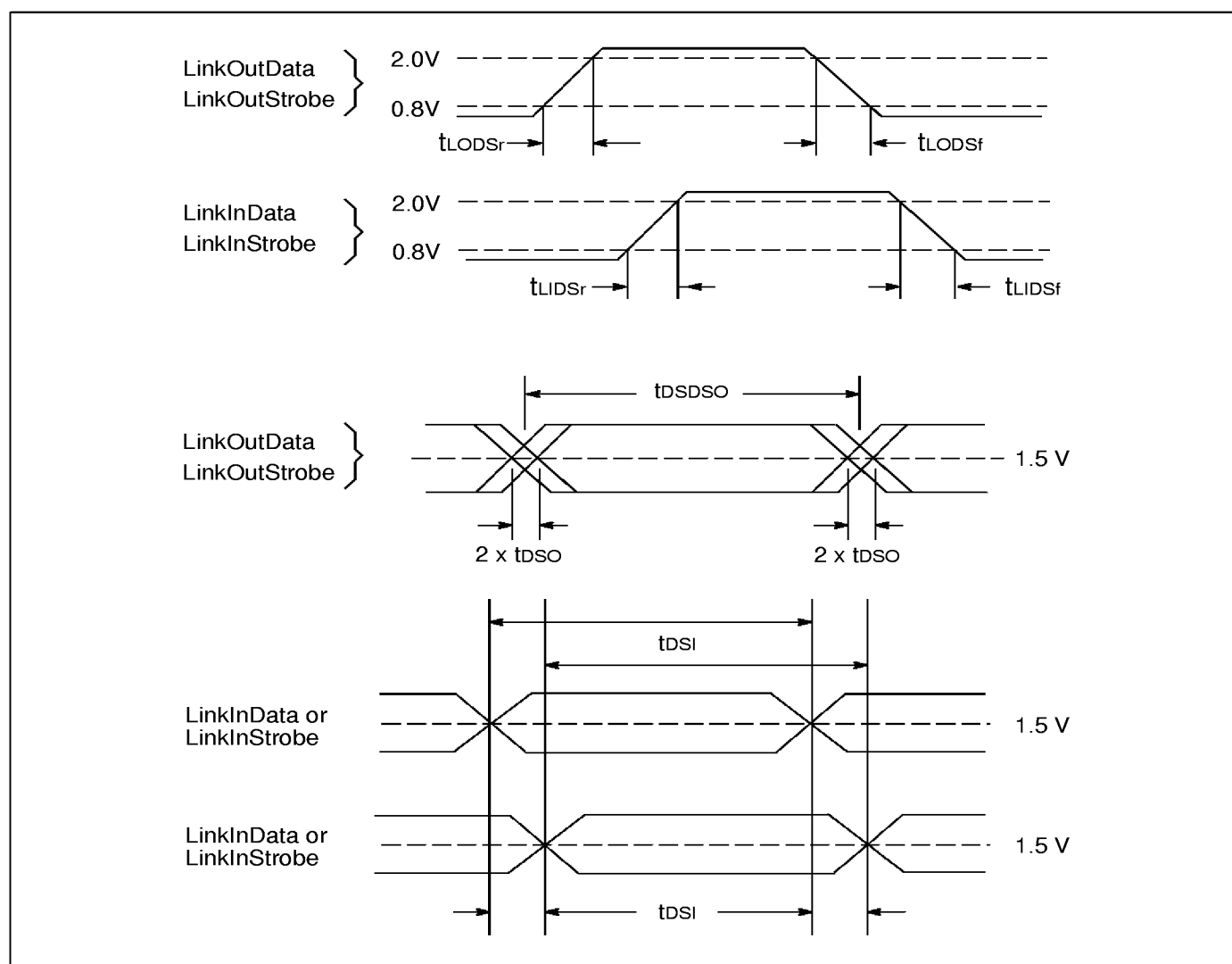
Figure 5.4 DS-Link timing
