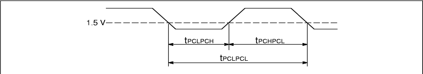
Figure 6.3 ProcClockOut timing
