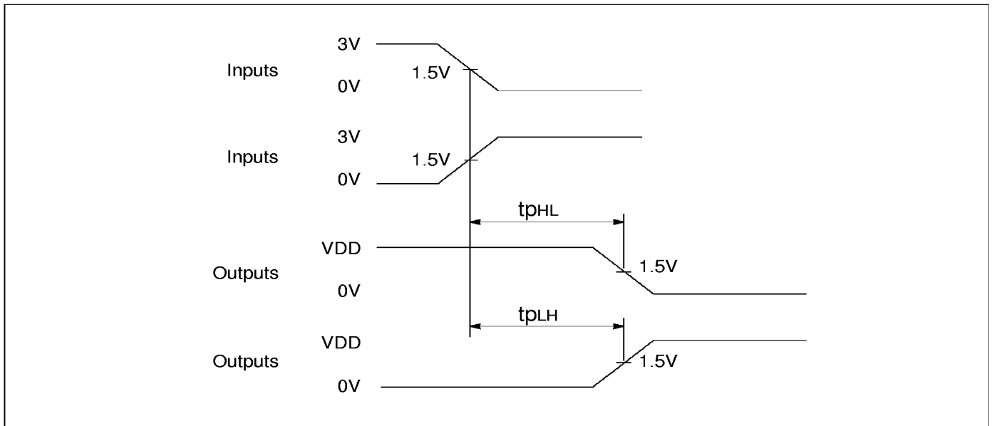
Figure 8.2 AC measurements timing waveforms
