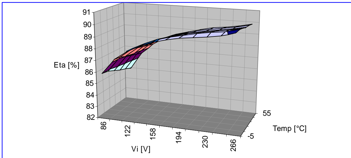
Figure 1. Efficiency vs. Input Voltage and Ambient Temperature, I_o = I_{o\ nom}
