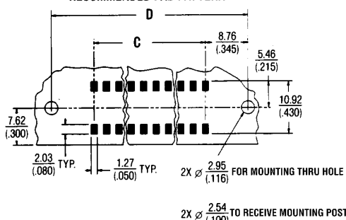
RECOMMENDED PAD PATTERN
