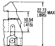
STYLE 2 CAT # 609-0004ES LATCH USED WITH STRAIN RELIEF
