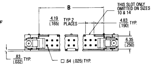
STYLE 1 CAT # 609-0004E LATCH USED W/O STRAIN RELIEF
