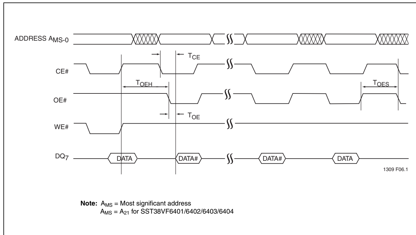
FIGURE 11: Data# Polling Timing Diagram
