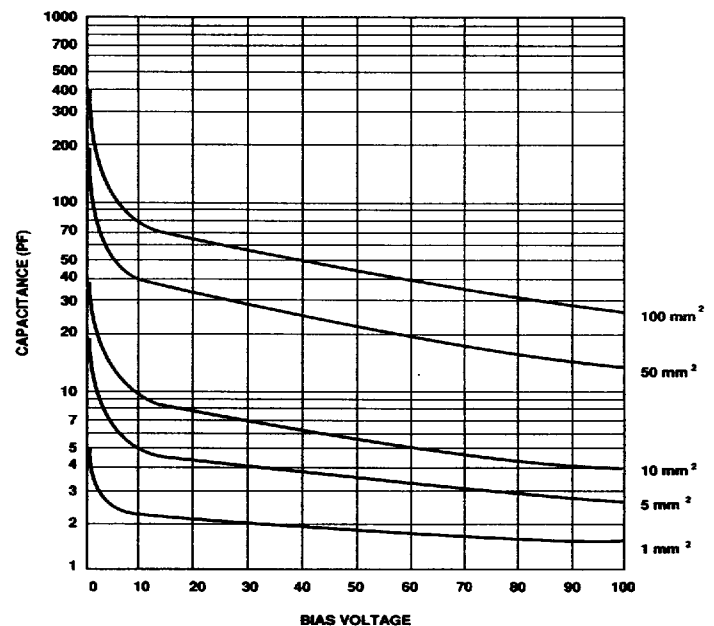
Fig.24 SERIES 4T - TYPICAL CAPACITANCE VERSUS BIAS VOLTAGE FOR A GIVEN DETECTOR AREA
