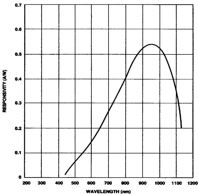
Fig.23 SERIES 4T - TYPICAL SPECTRAL RESPONSE
