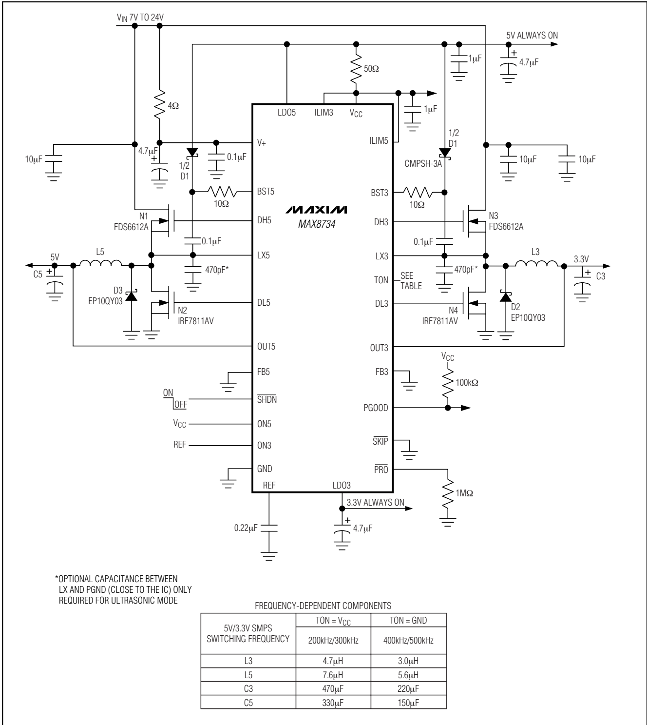
Figure 2. MAX8734 Typical Application Circuit
