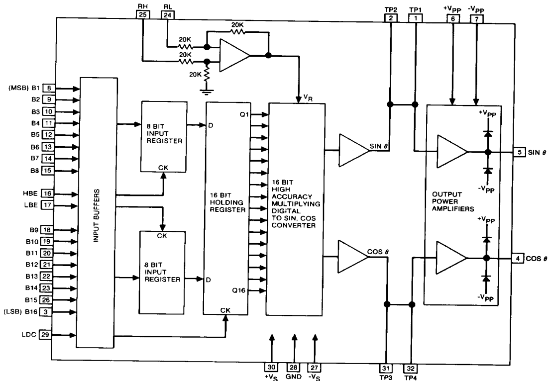
FIGURE 1 2106 Block Diagram
