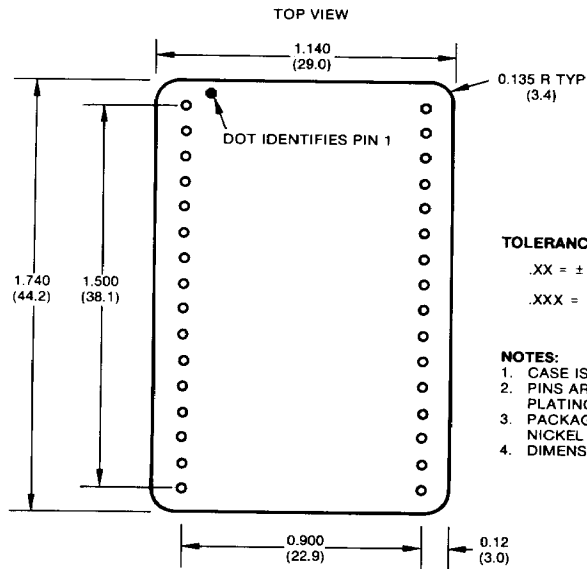
MECHANICAL OUTLINE (32 PIN TRIPLE DIP)
