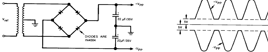
FIGURE 8 Pulsating Power Supply
