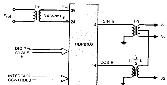
FIGURE 12 Digital-to-Synchro Converter
