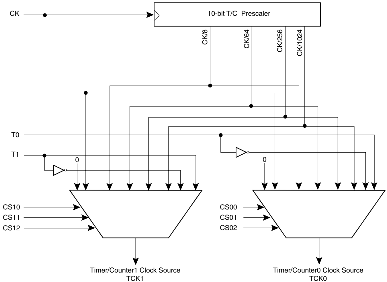
Figure 12. Timer/Counter Prescaler
