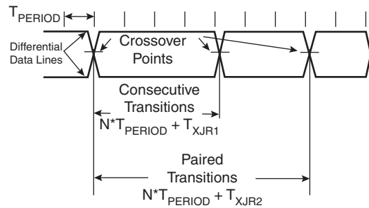
Figure 31. Differential Data Jitter
