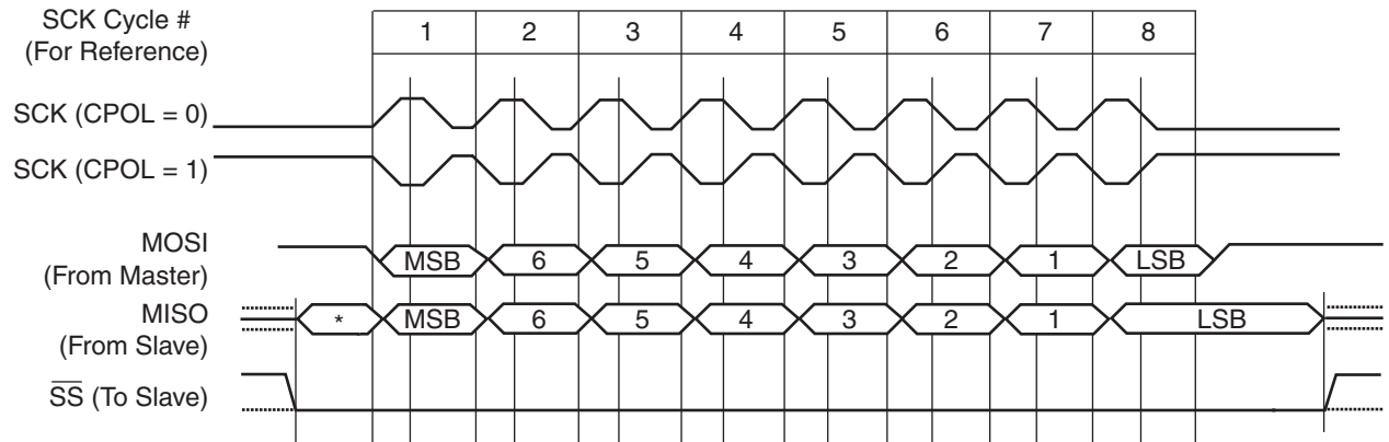
Figure 21. SPI Transfer Format with CPHA = 1 and DORD = 0
