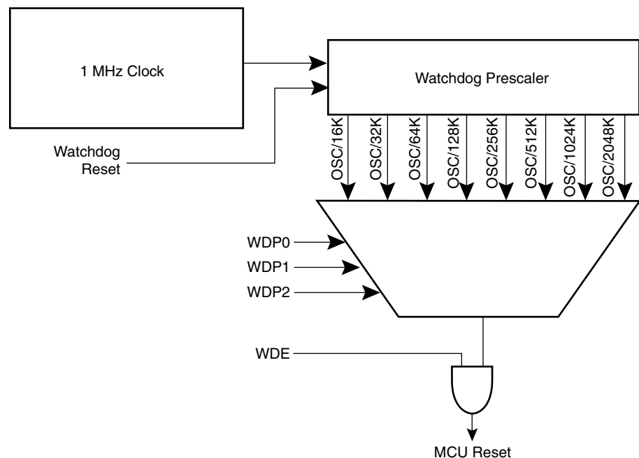
Figure 17. Watchdog Timer
