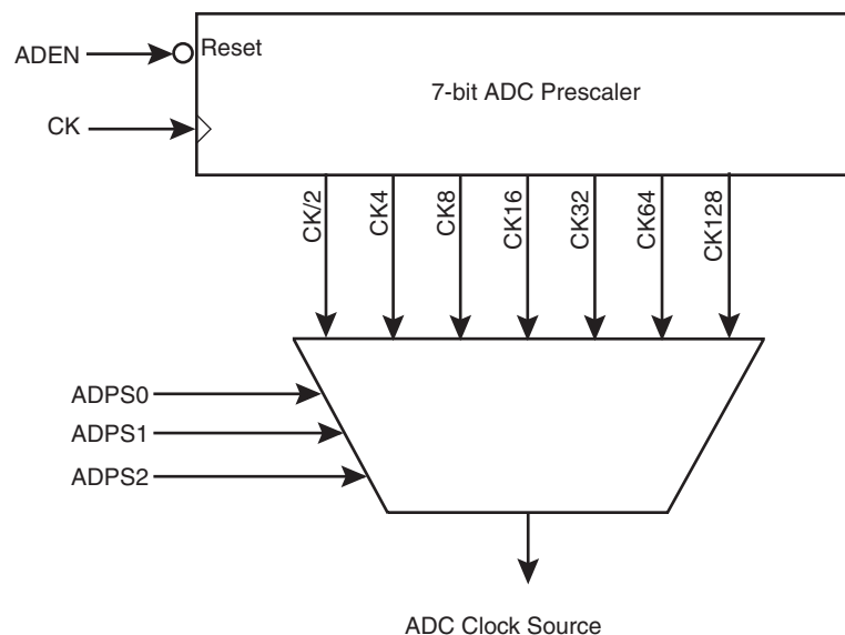
Figure 23. ADC Prescaler
