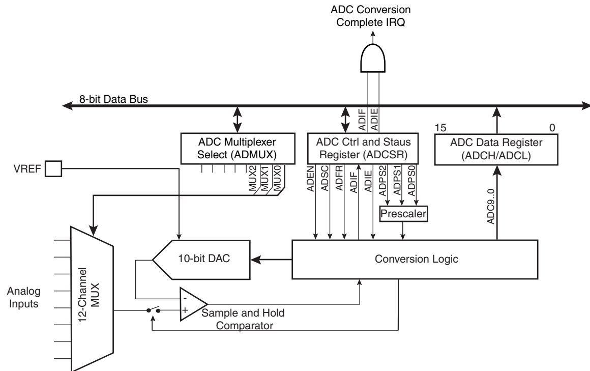
Figure 22. Analog-to-digital Converter Block Schematic
