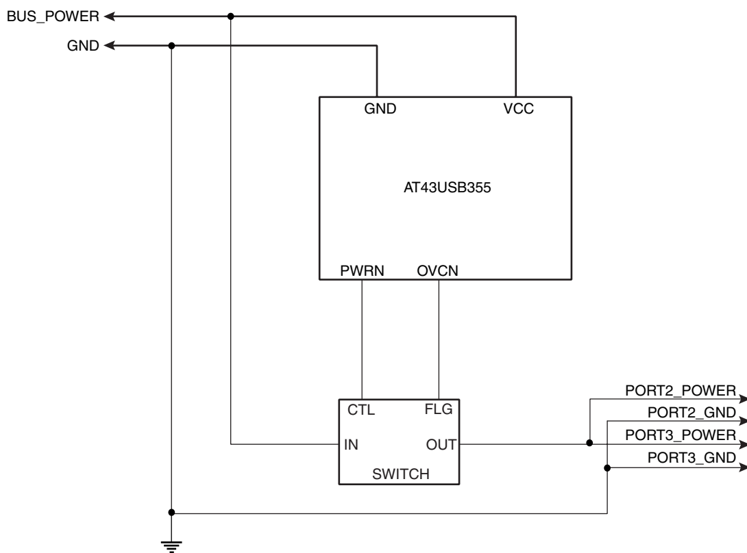
Figure 27. Port Power Management
