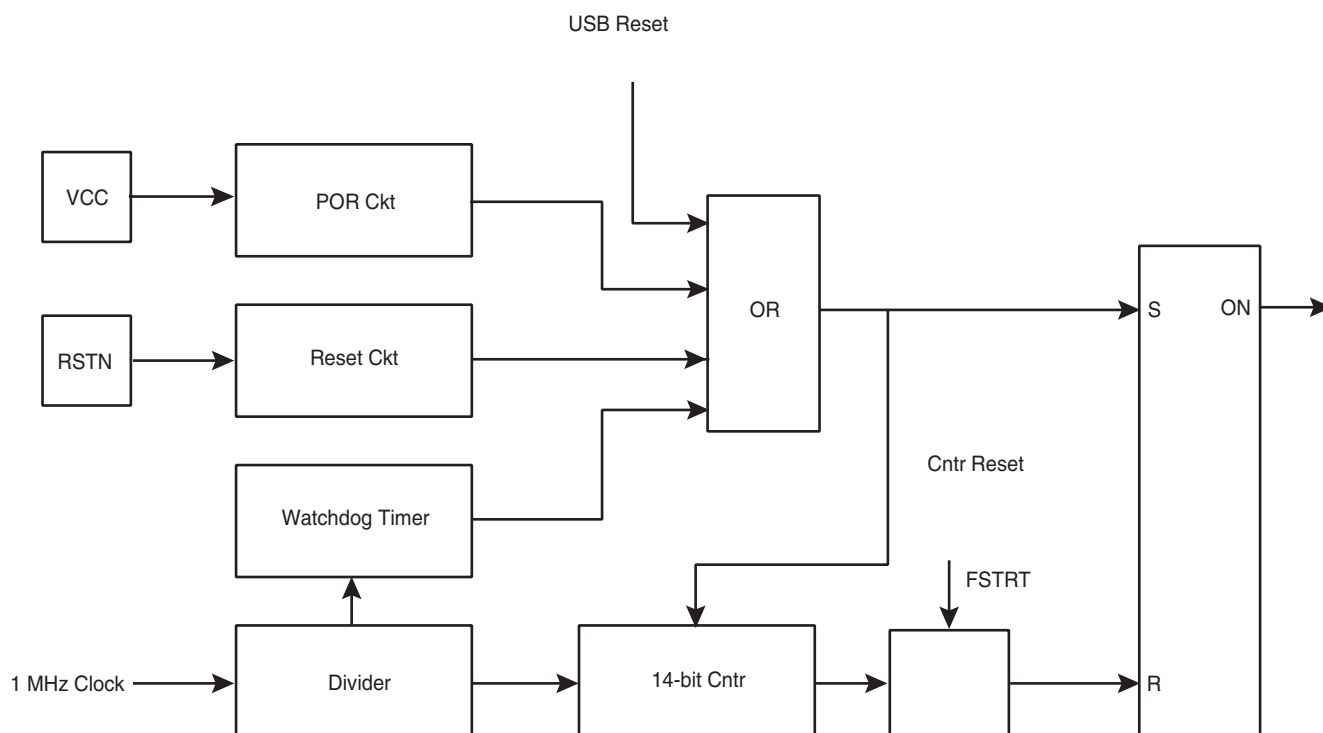
Figure 9. Reset Logic
