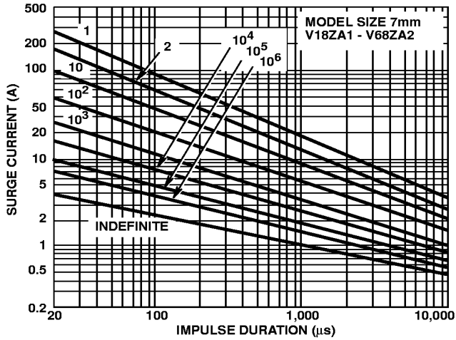
FIGURE 18. SURGE CURRENT RATING CURVES FOR V18ZA1 - V68ZA2
