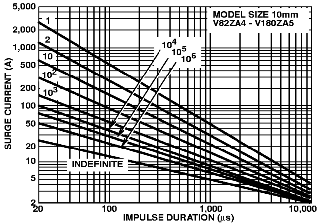
FIGURE 22. SURGE CURRENT RATING CURVES FOR V82ZA4 - V180ZA5
