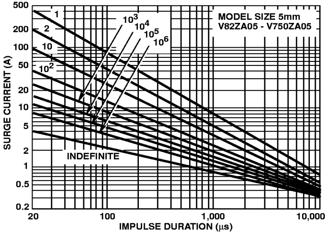
FIGURE 16. SURGE CURRENT RATING CURVES FOR V82ZA05 - V750ZA05
