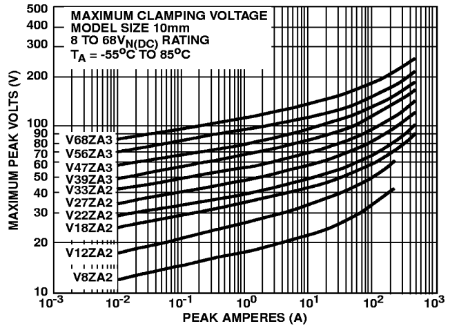
FIGURE 8. CLAMPING VOLTAGE FOR V8ZA2 - V68ZA3
