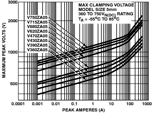
FIGURE 5. CLAMPING VOLTAGE FOR V360ZA05 - V750ZA05
