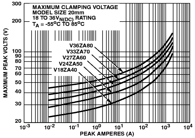
FIGURE 12. CLAMPING VOLTAGE FOR V18ZA40 - V36ZA80
