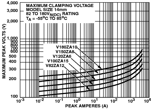
FIGURE 11. CLAMPING VOLTAGE FOR V82ZA12 - V180ZA10
