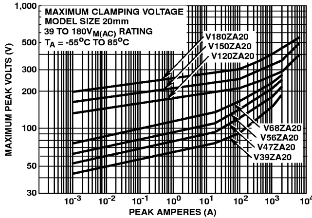
FIGURE 13. CLAMPING VOLTAGE FOR V39ZA20 - V180ZA20
