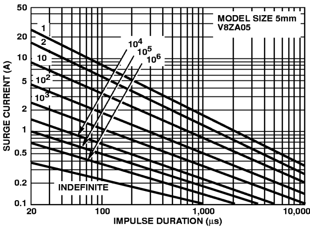
FIGURE 14. SURGE CURRENT RATING CURVES FOR V8ZA05
