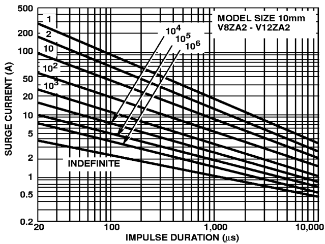
FIGURE 20. SURGE CURRENT RATING CURVES FOR V8ZA2 - V127ZA2
