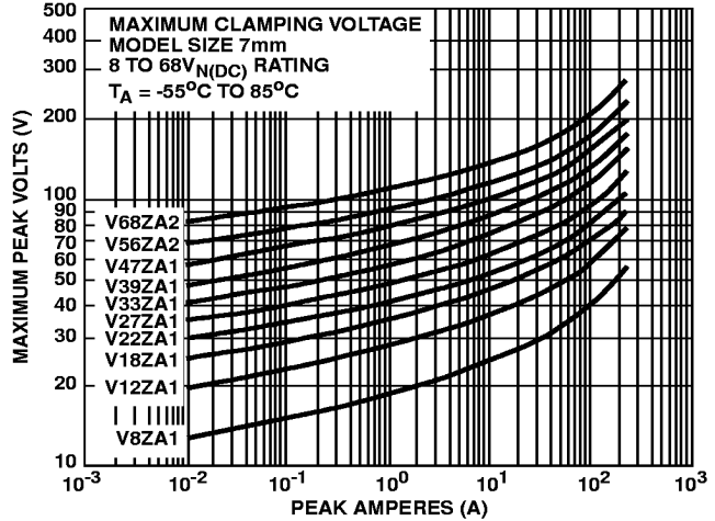
FIGURE 6. CLAMPING VOLTAGE FOR V8ZA1 - V68ZA2
