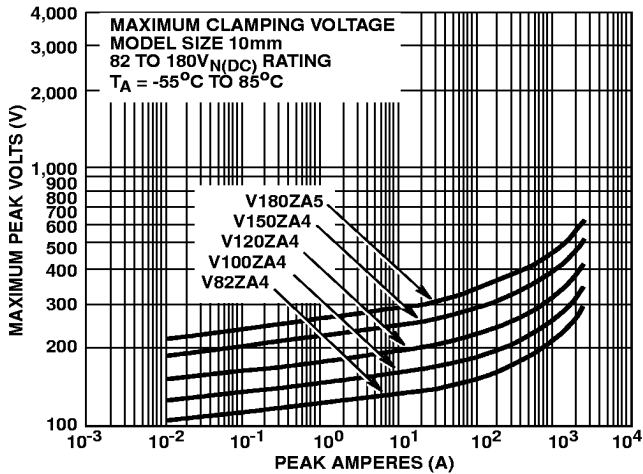
FIGURE 9. CLAMPING VOLTAGE FOR V82ZA4 - V180ZA5
