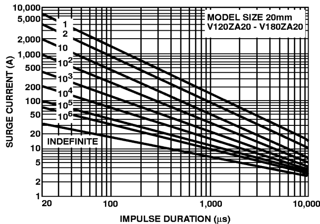
FIGURE 26. SURGE CURRENT RATING CURVES FOR V120ZA20 - V180ZA20
