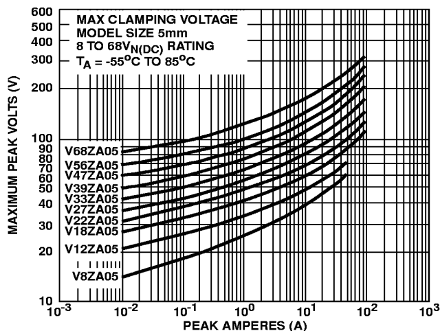
FIGURE 3. CLAMPING VOLTAGE FOR V8ZA05 - V68ZA05
