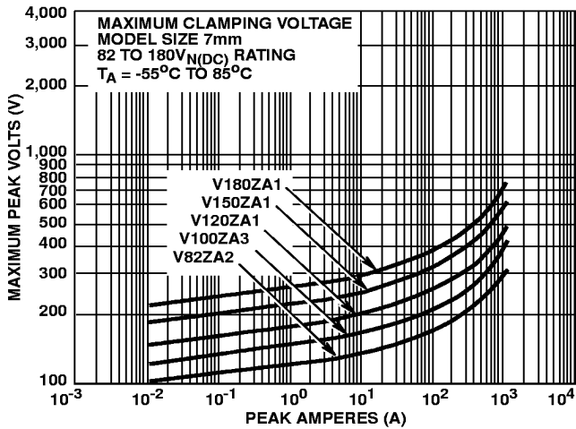
FIGURE 7. CLAMPING VOLTAGE FOR V82ZA2 - V180ZA1
