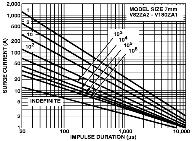
FIGURE 19. SURGE CURRENT RATING CURVES FOR V82ZA2 - V180ZA1
