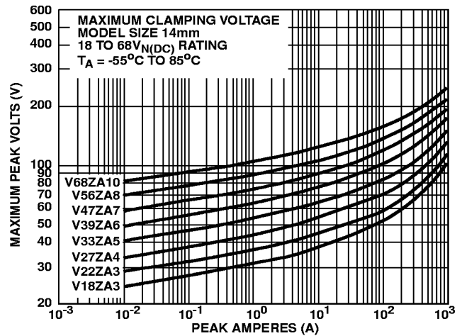
FIGURE 10. CLAMPING VOLTAGE FOR V18ZA3 - V68ZA10
