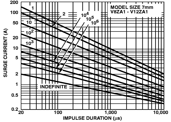
FIGURE 17. SURGE CURRENT RATING CURVES FOR V8ZA1 - V12ZA1
