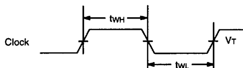
Clock Width
