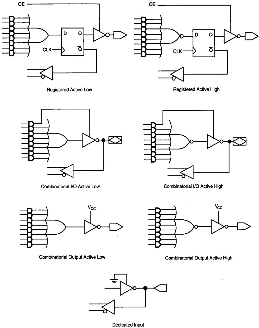
Figure 2. Macrocell Configurations
