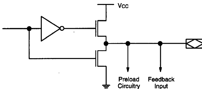
Typical Output
