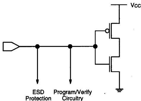
Typical Input
