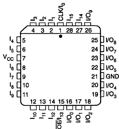
PLCC
