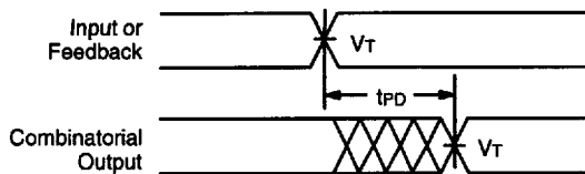
Combinatorial Output
