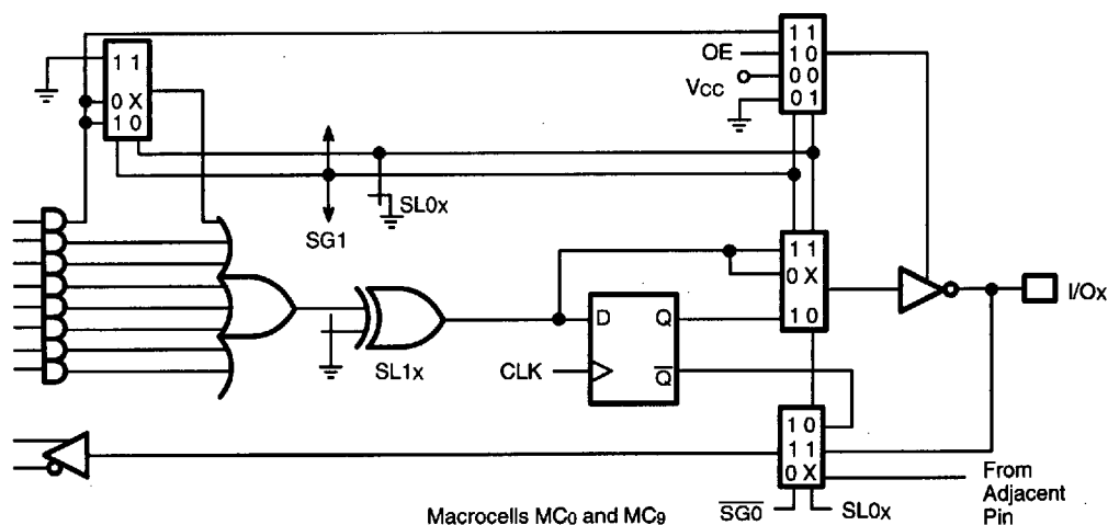
PALCE24V10 Macrocell
