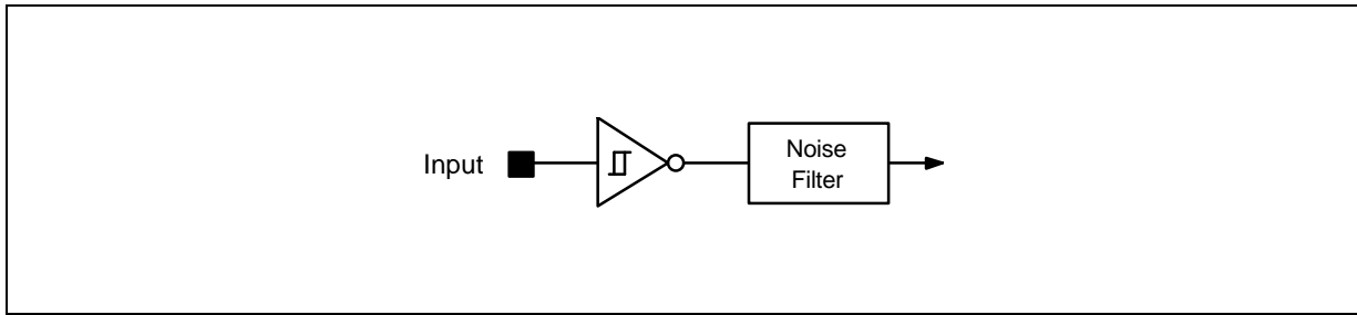
Figure 1-3. Pin Circuit Type 1 (V-Sync H-Sync, CAPA)
