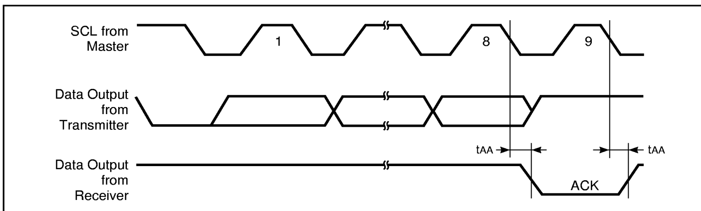
Figure 2. ACKnowledge Response from Receiver
