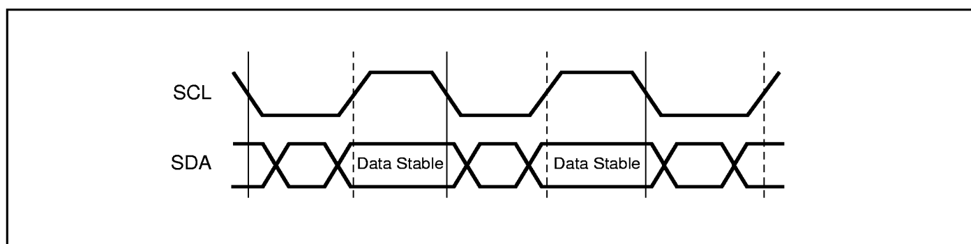
Figure 4. Data Validity Protocol
