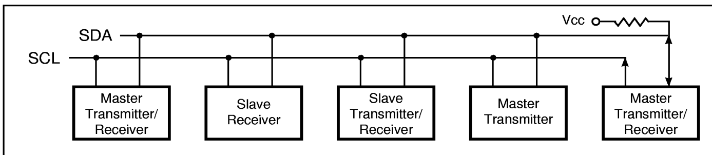
Figure 1. Typical System Bus Configuration
