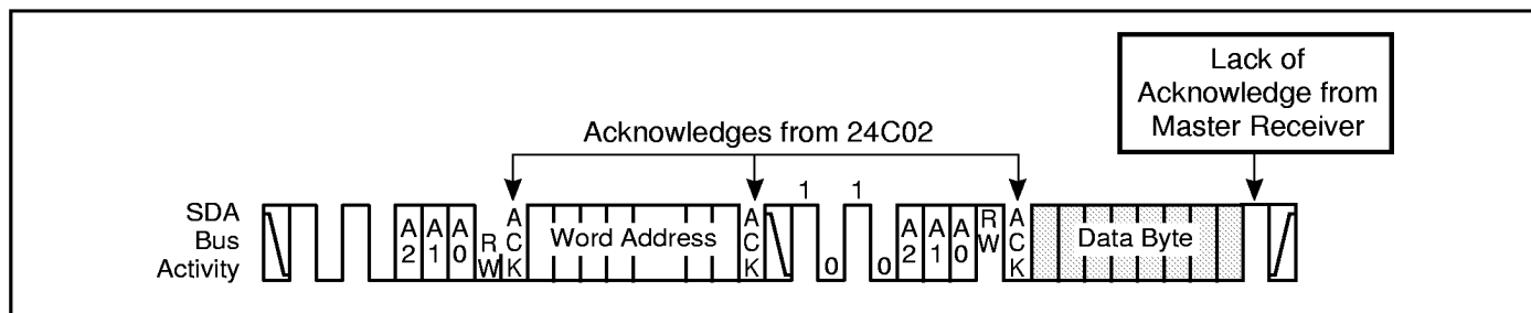
Figure 8. Random Access Read
