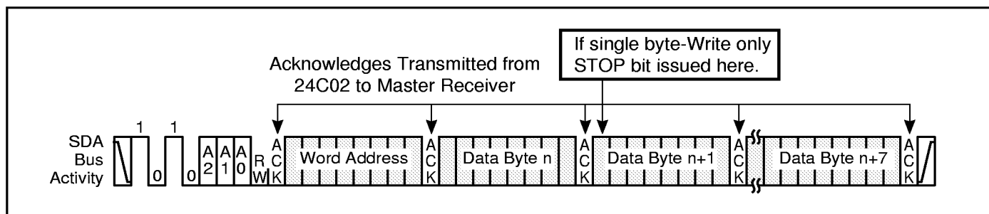
Figure 6. Write Operation
