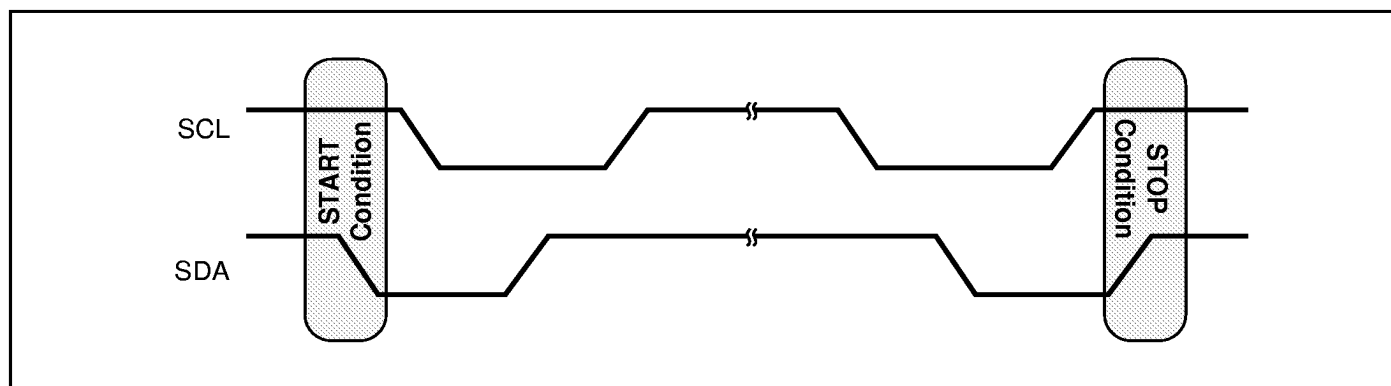
Figure 3. START and STOP Conditions
