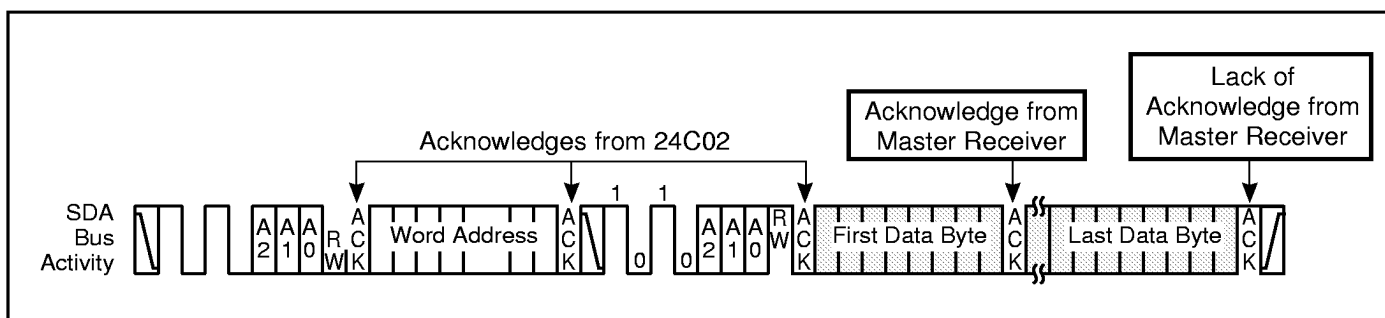
Figure 9. Sequential Read
