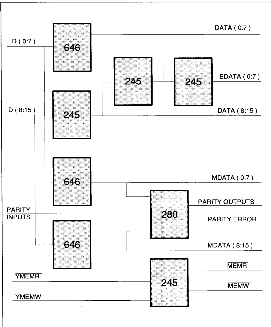
FIGURE 1-2. FE3031 FUNCTIONAL BLOCK DIAGRAM
