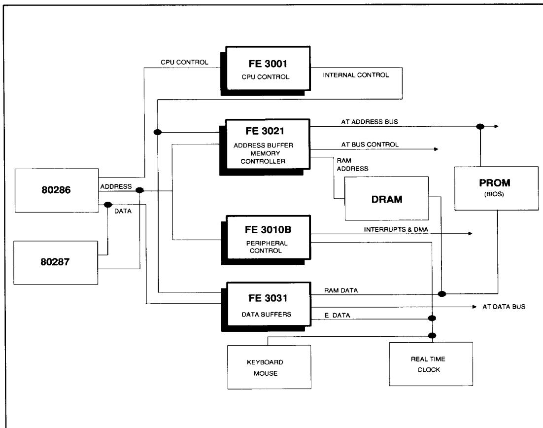
FIGURE 1-1. FE3600B CHIP SET FUNCTIONAL BLOCK DIAGRAM
