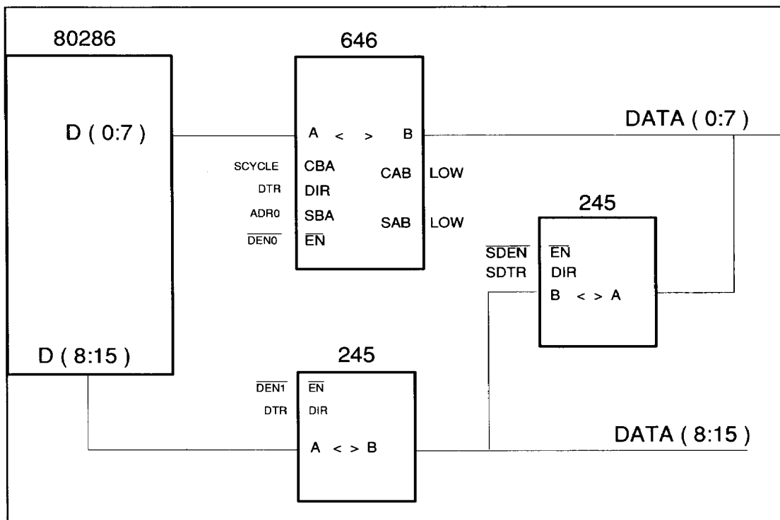
FIGURE 6-1. PC/AT DATA BUS ARCHITECTURE
